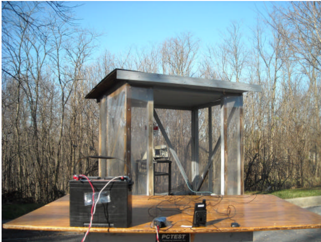
Figure 1-5 iFMCLA Set-up – Test Configuration #5
