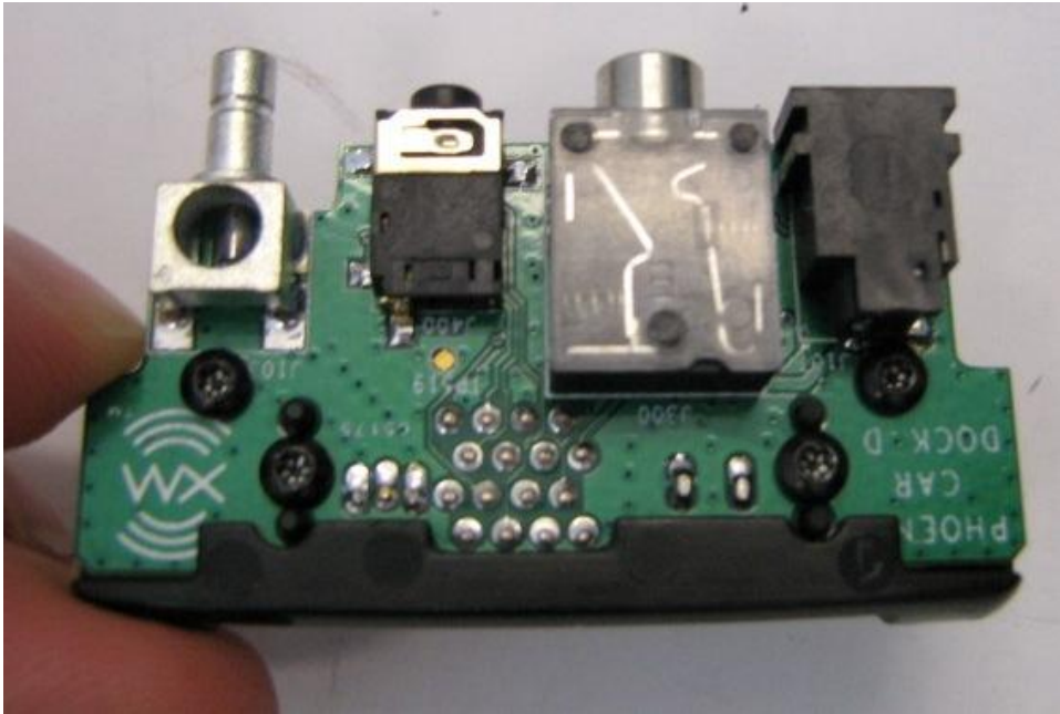
Back of PCB
