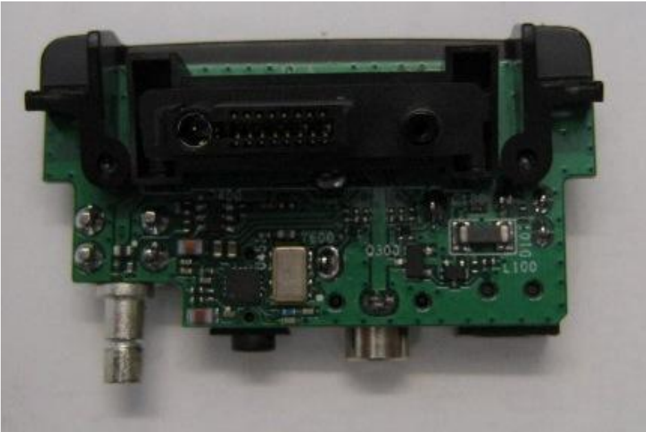
Front of PCB
