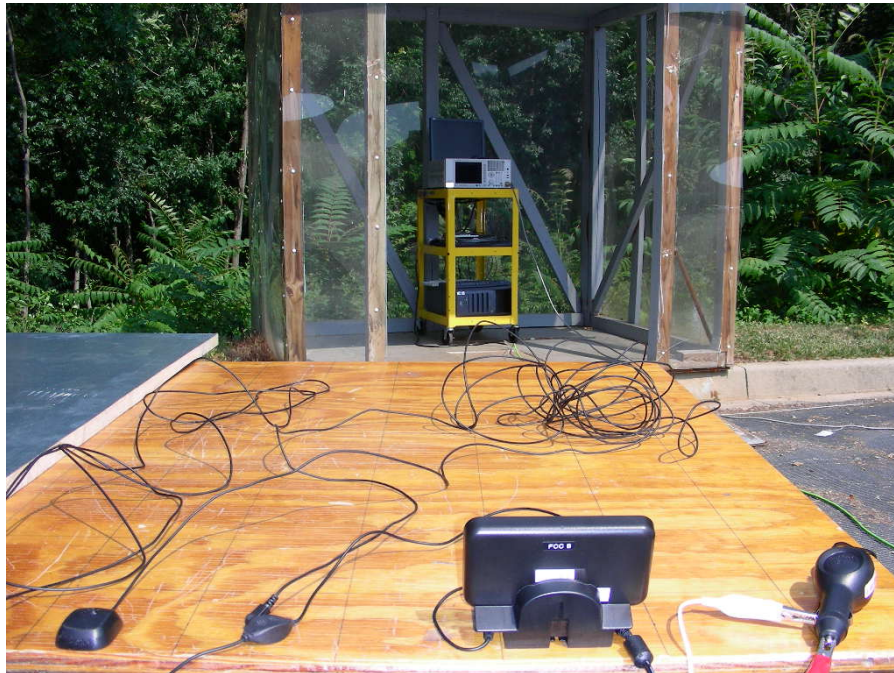
Figure 1-6. SureConnect with FM Antenna Set-up – Test Configuration #6
