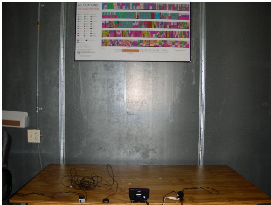
Figure 1-2. 20dB Bandwidth Set-up – Test Configuration #5
