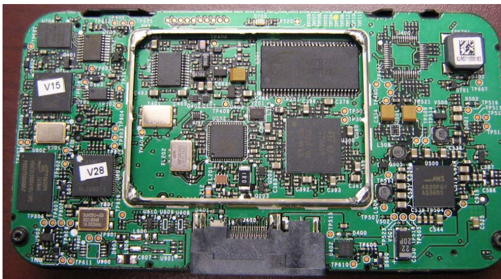
Back of PCB no shield
