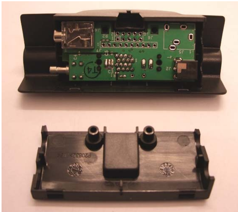
Open Car Cradle with PCB
