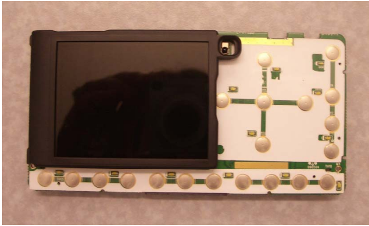
Front View PCBA (with LCD/Frame/Snubber)
