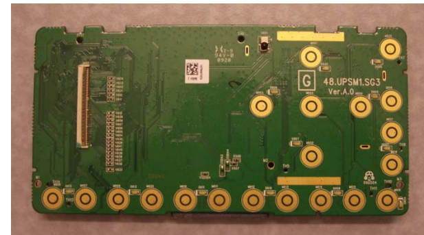
Front View PCBA (with Popple Domes Removed)
