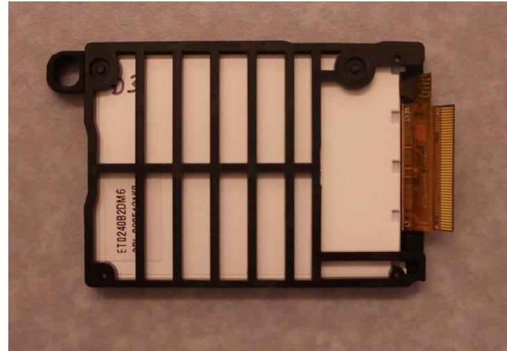
Back View of LCD/ Frame/Snubber
