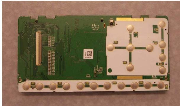
Front View PCBA
