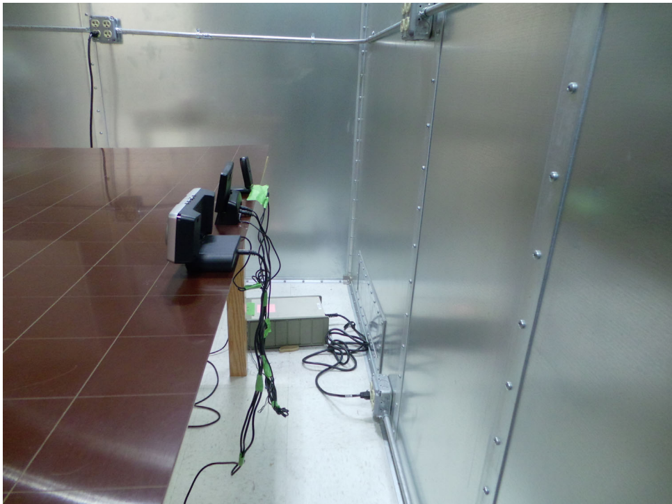
Test Configuration 1: Conducted Emissions, Endeavor with Home Cradle (side)
