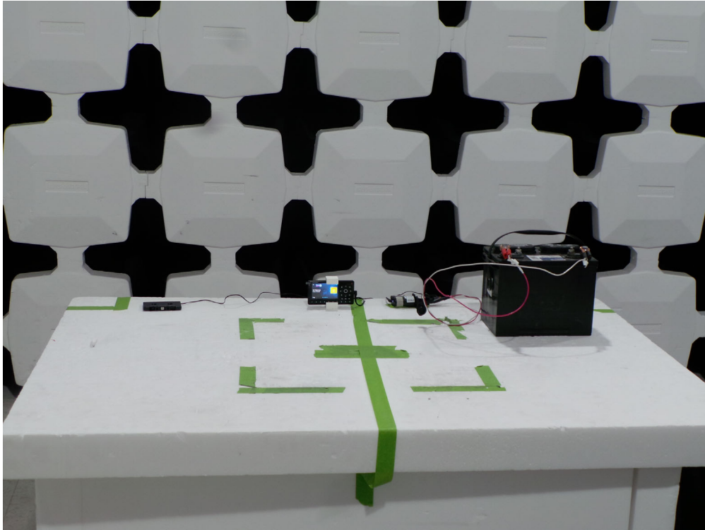
Configuration 2: Rody BT Radio with Cassette Adapter (front)
