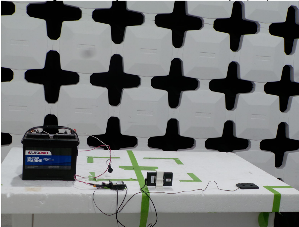
Configuration 2: Rody BT Radio with Cassette Adapter (rear)
