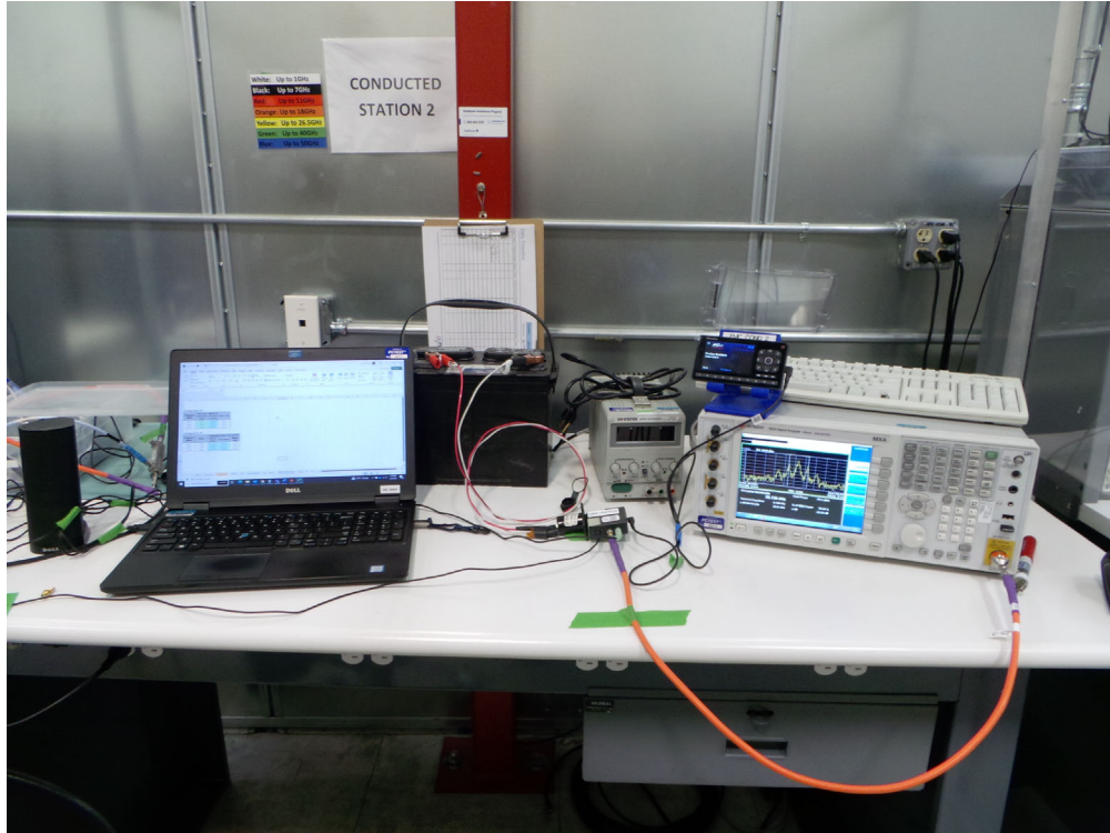
Configuration 3 & 4: Rody BT, FM Conducted Measurements
