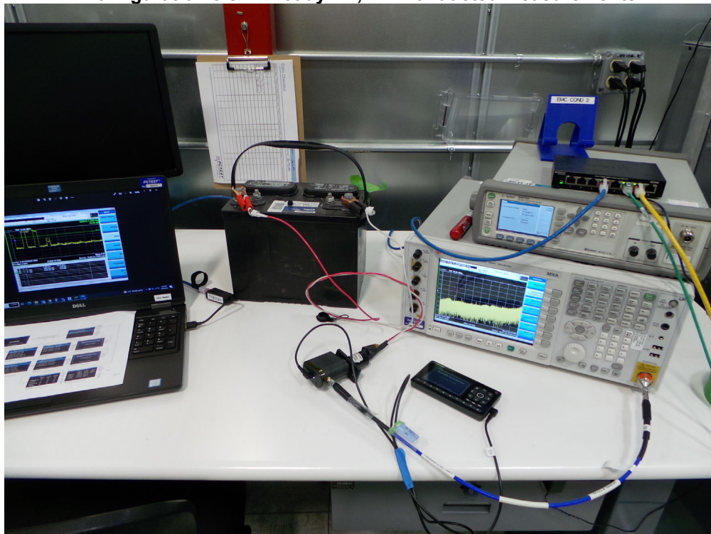
Configuration 5: Rody BT, Bluetooth Mode
