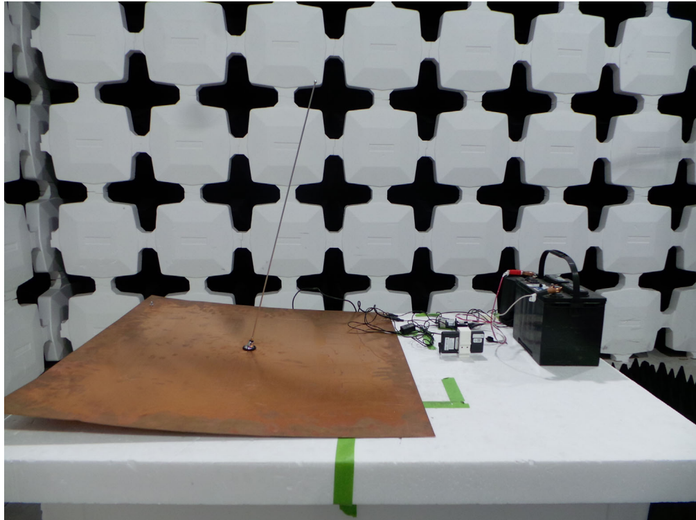
Configuration 1: Rody BT Radio with FM Direct Adapter(FMDA25) (front)
