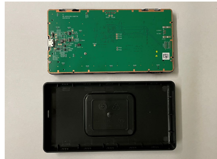
Rear View with Rear Cover Removed
