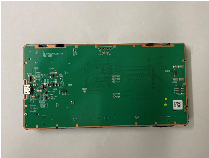
PCBA Rear View (w/front housing & screws)
