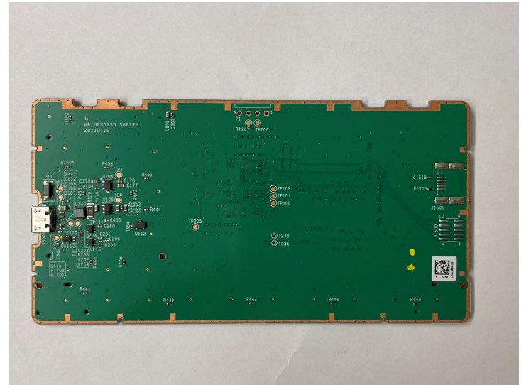
PCBA Rear View (no housing or screws)
