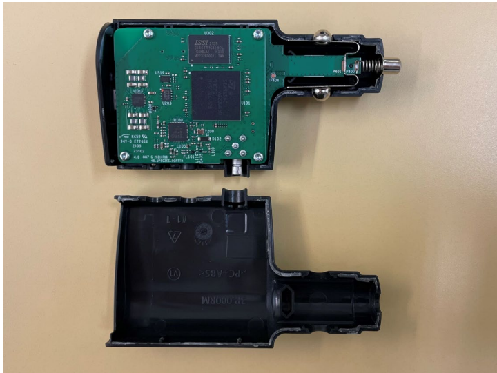
PCBAs Right View (w/housings & screws)
