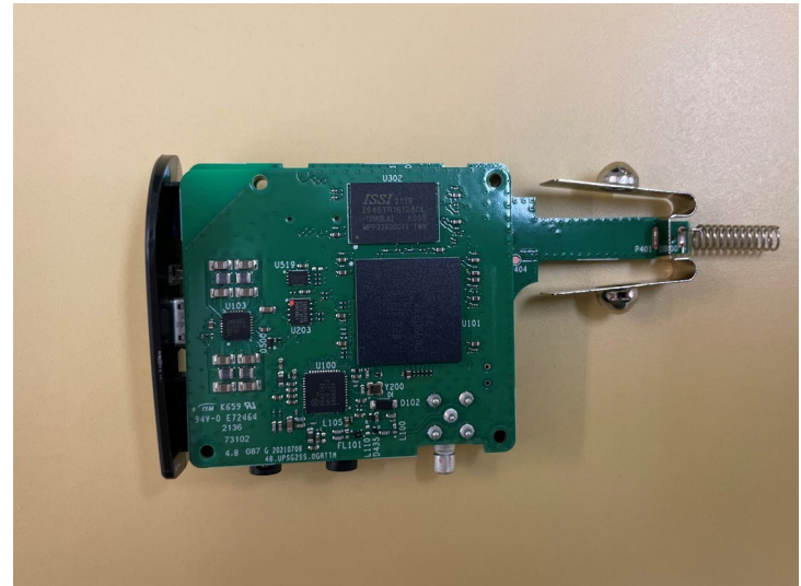
PCBAs Right View (no side housings or screws)
