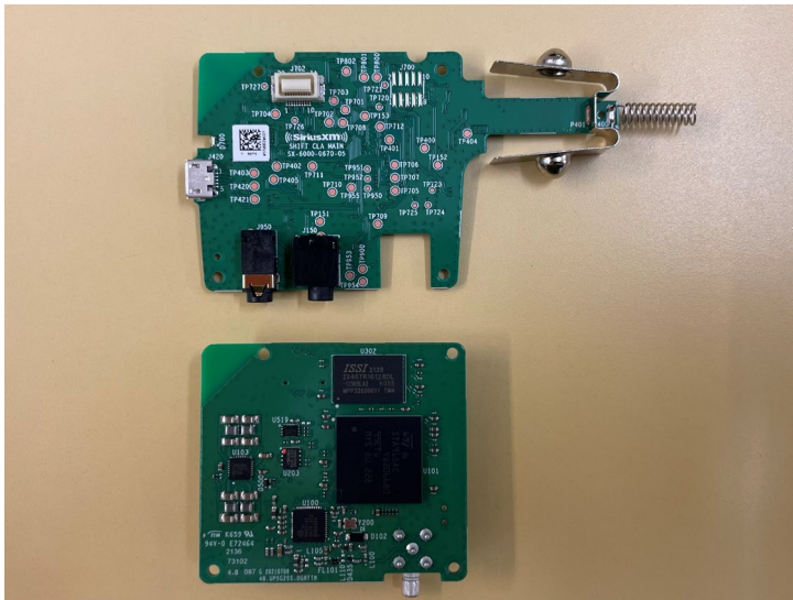
PCBAs Right View (no housings)
