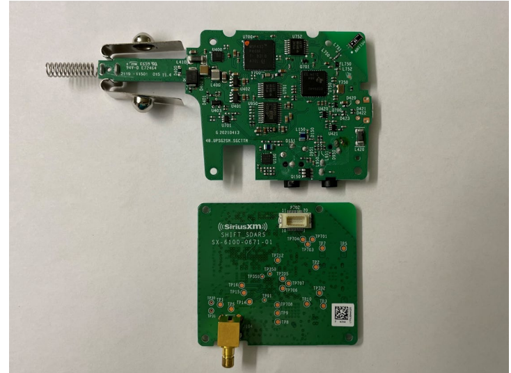
PCBAs Left View (no housings)
