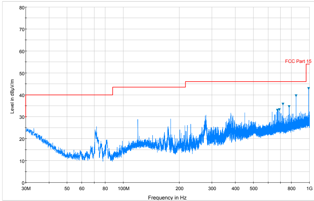
7-5. Radiated Spurious Plot below 1GHz (Configuration #3, Pol. H)
