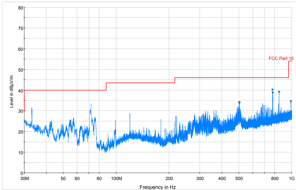
7-6. Radiated Spurious Plot below 1GHz (Configuration #3, Pol. V)
