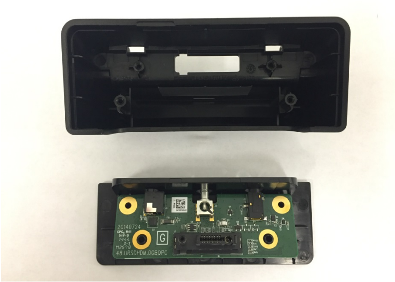
Top and Bottom Housing with PCBA
