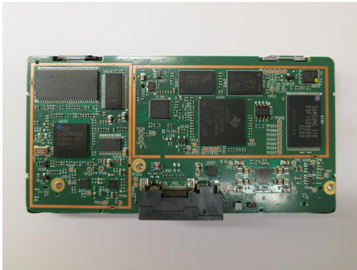
PCBA Rear View (w/rear housing & screws)
