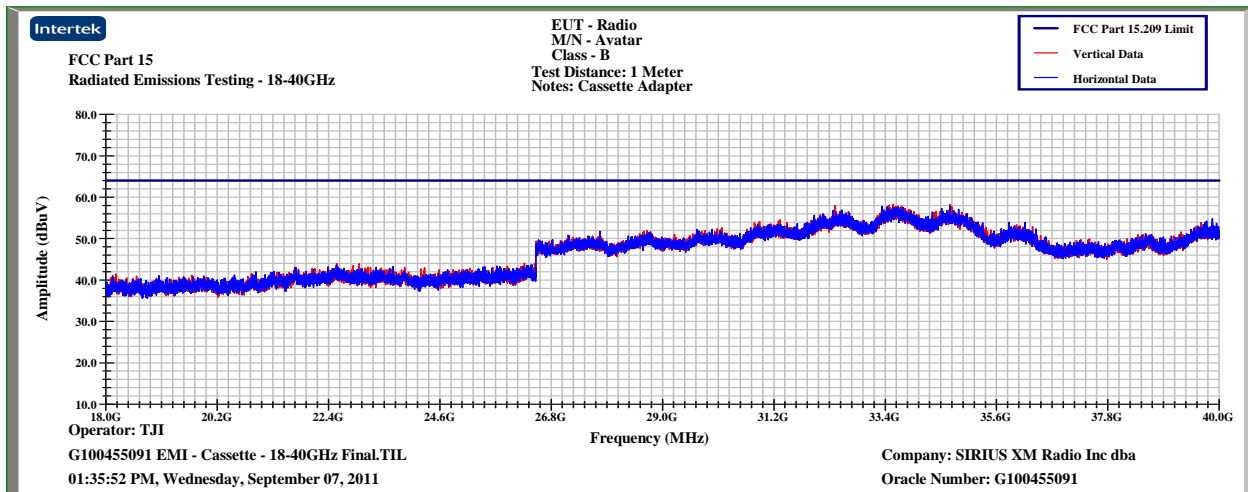
Peak Plot – 18000MHz-40000MHz
