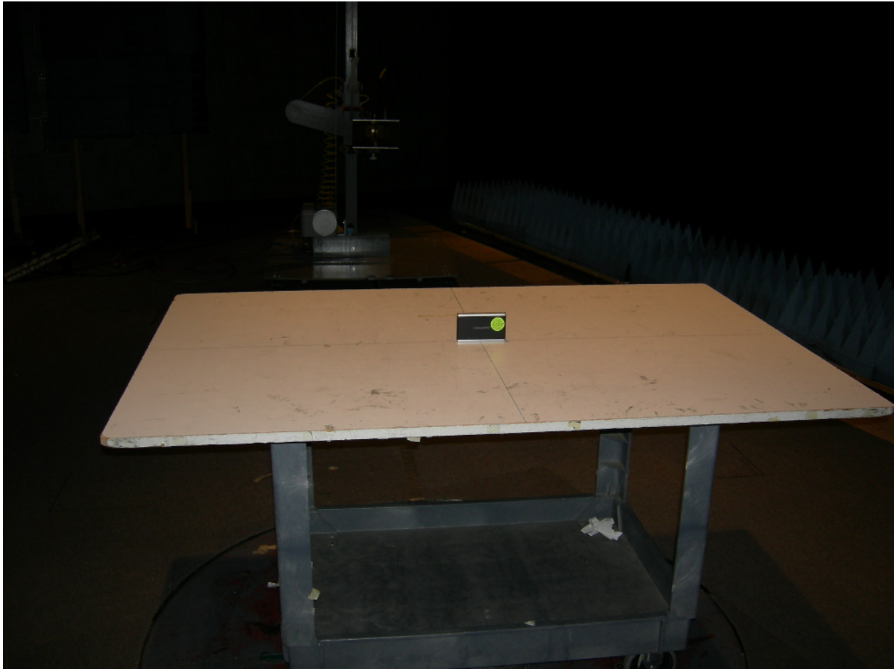
Figure 4: Test Setup – Y Orientation
