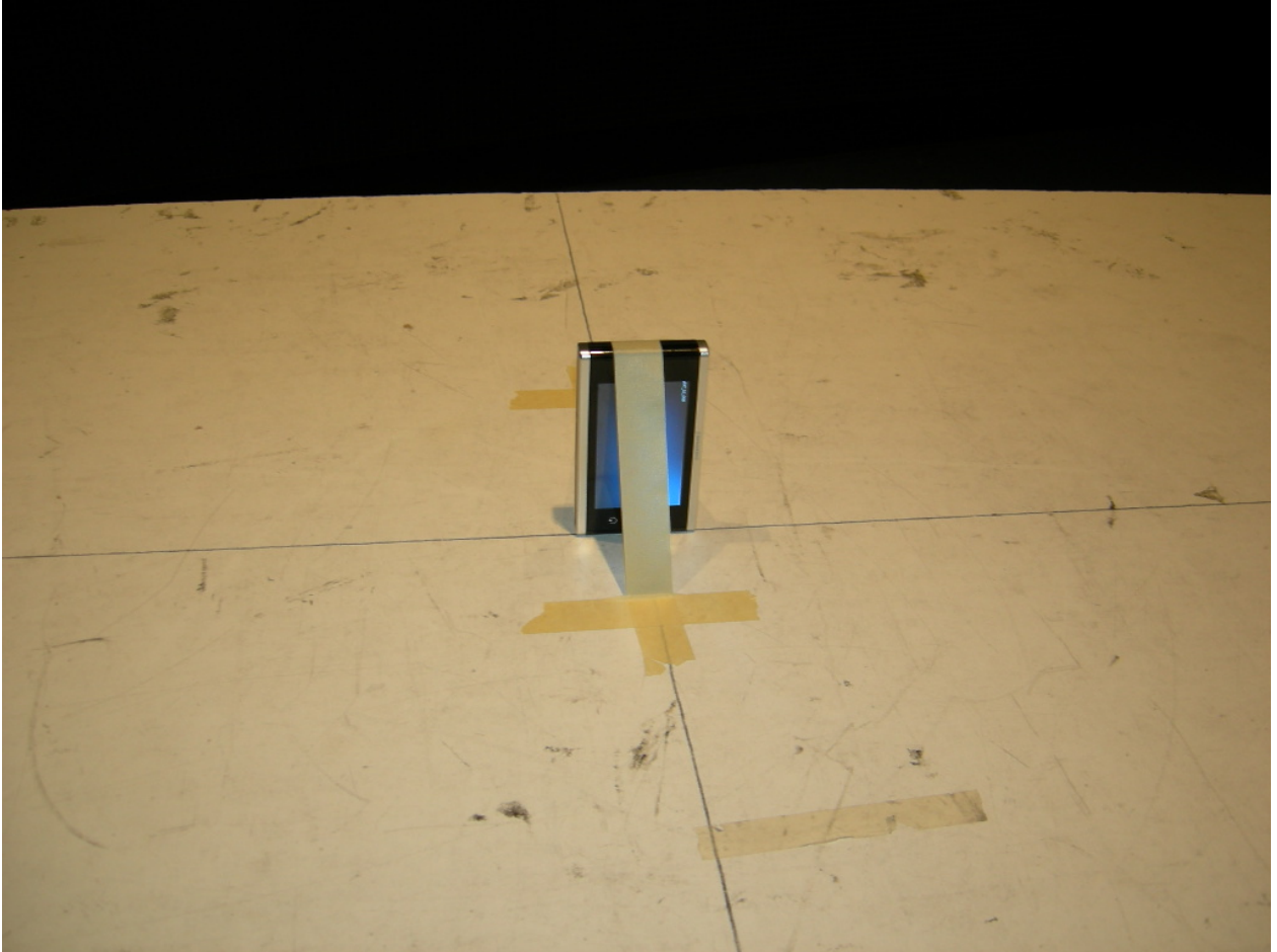
Figure 5: Test Setup – Z Orientation
