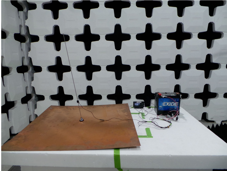
Configuration 9: Onyx EZR with Xpress Car Dock & SureConnect Adapter (front)
