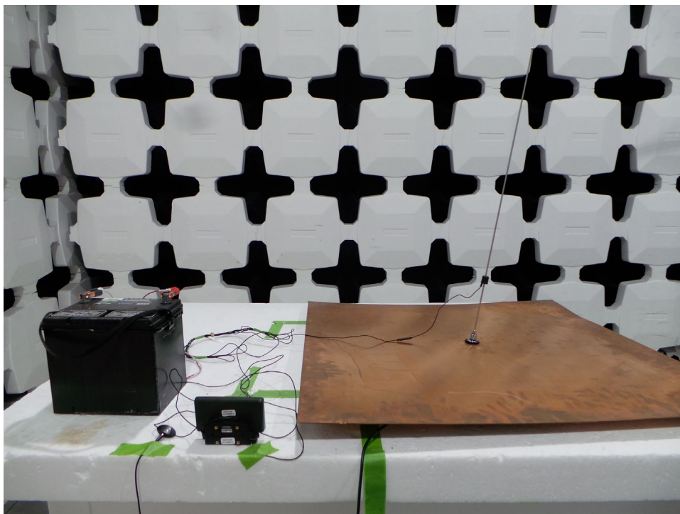
Configuration 9: Onyx EZR with Xpress Car Dock & SureConnect Adapter (rear)
