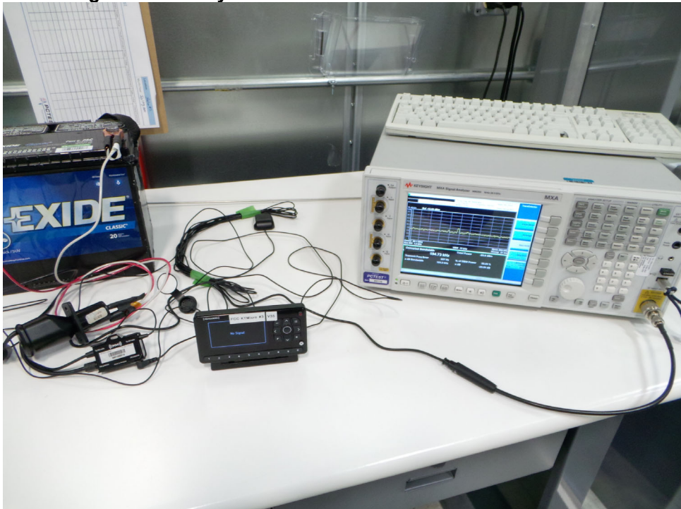
Configuration 6: Onyx EZR with Xpress Car Dock & FM Direct Adapter (XMFM1)
