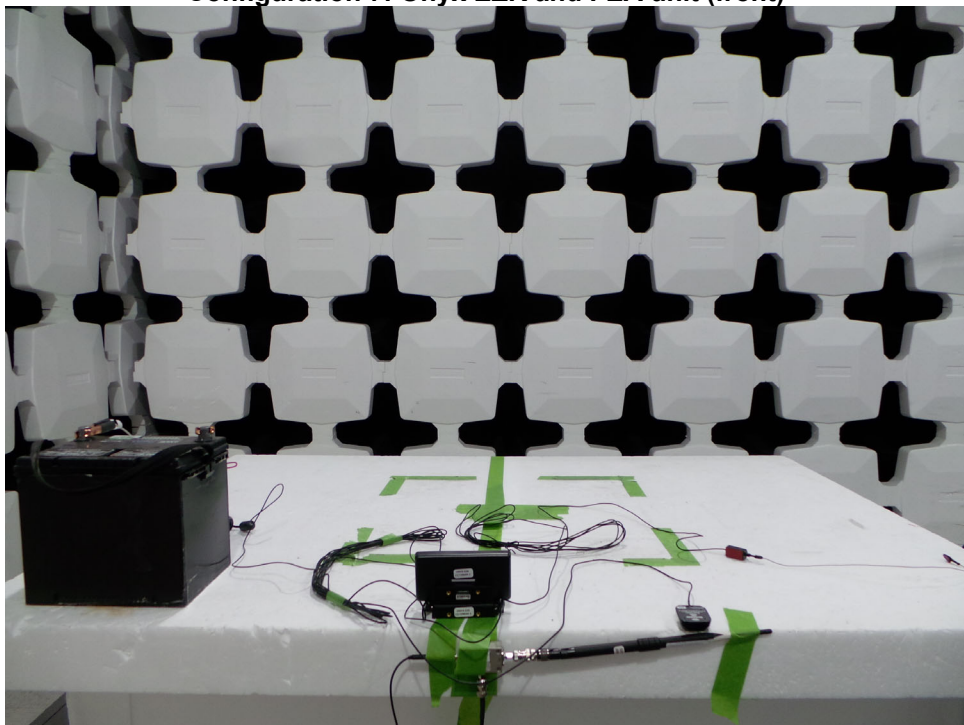
Configuration 7: Onyx EZR and FEA unit (rear)
