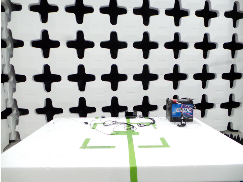
Configuration 7: Onyx EZR and FEA unit (front)
