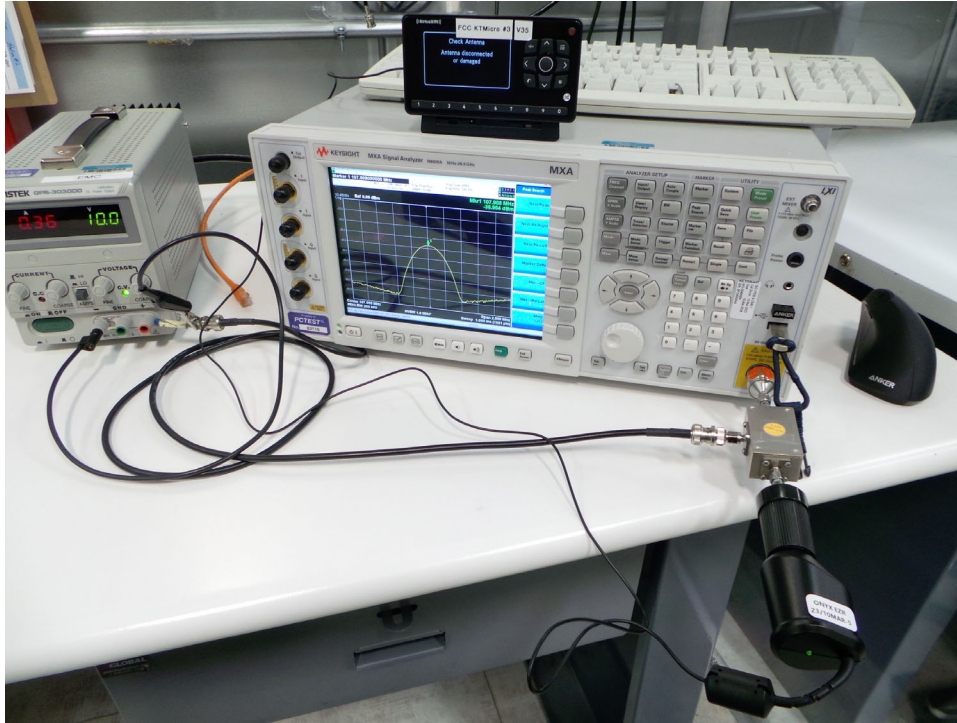
Configuration 10: Onyx EZR with Bias-Tee
