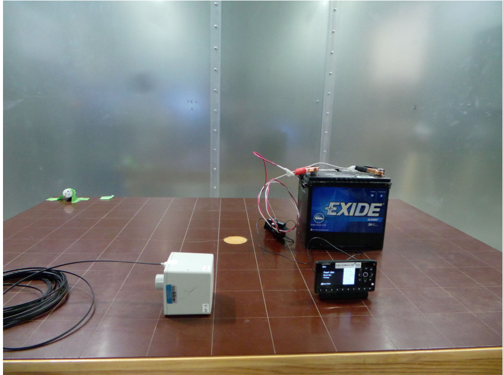
Configuration 11: Onyx EZR Receiver with Power Connect
