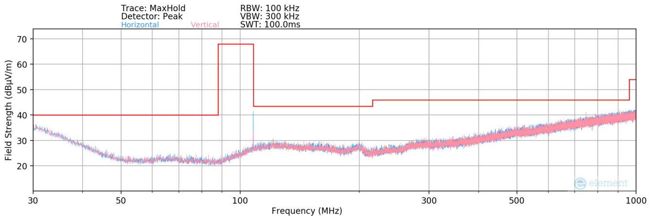
Plot 8-12. Radiated Spurious Plot below 1GHz (107.9MHz Configuration #7)
