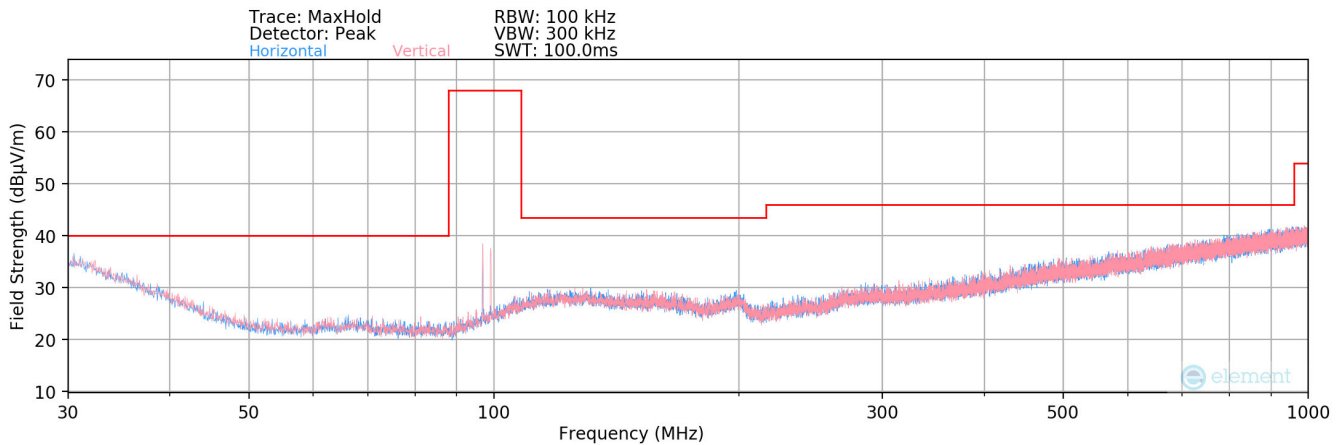
Plot 8-14. Radiated Spurious Plot below 1GHz (96.9MHz Configuration #8)
