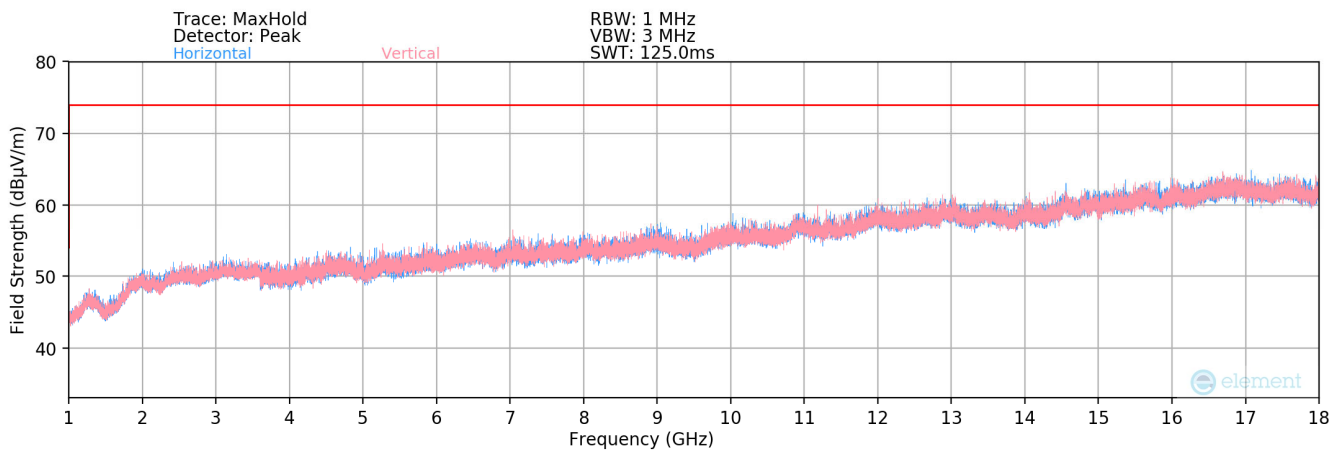
Plot 8-20. Radiated Spurious Plot above 1GHz (96.9MHz)
