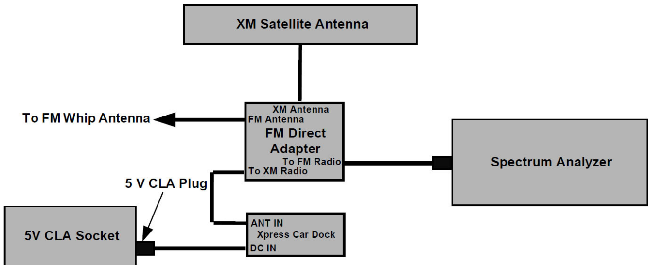
Figure 8-2. Test Instrument & Measurement Setup (Configuration #6 XpressCar Dock & FM Direct Adapter)
