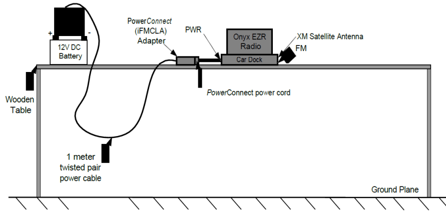
Figure 8-10. Test Instrument & Measurement Setup (Configuration #8 PowerConnect only)
