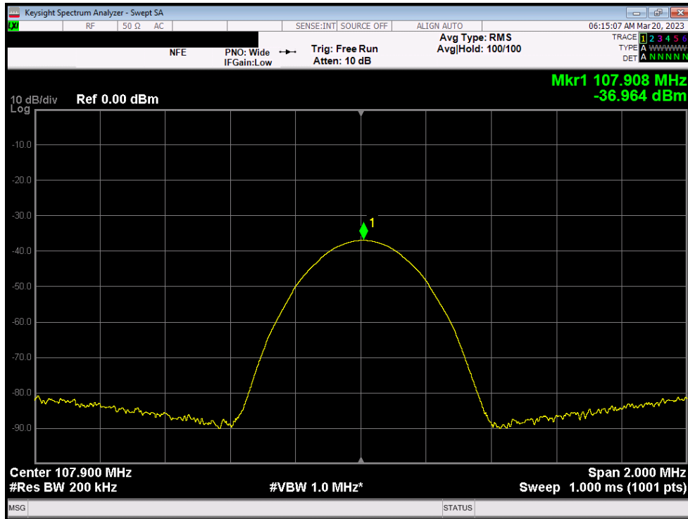
Plot 8-9. Peak Conducted Power (High Channel – 107.9MHz)
