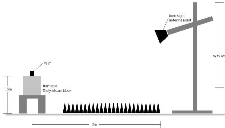
Figure 8-8. Test Instrument & Measurement Setup
