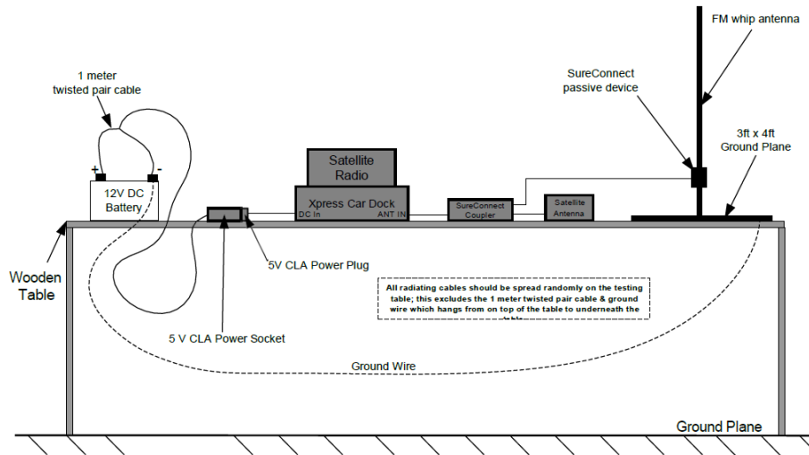
Figure 8-11. Test Instrument & Measurement Setup (Configuration #9 Xpress Car Dock & SureConnect Adapter)
