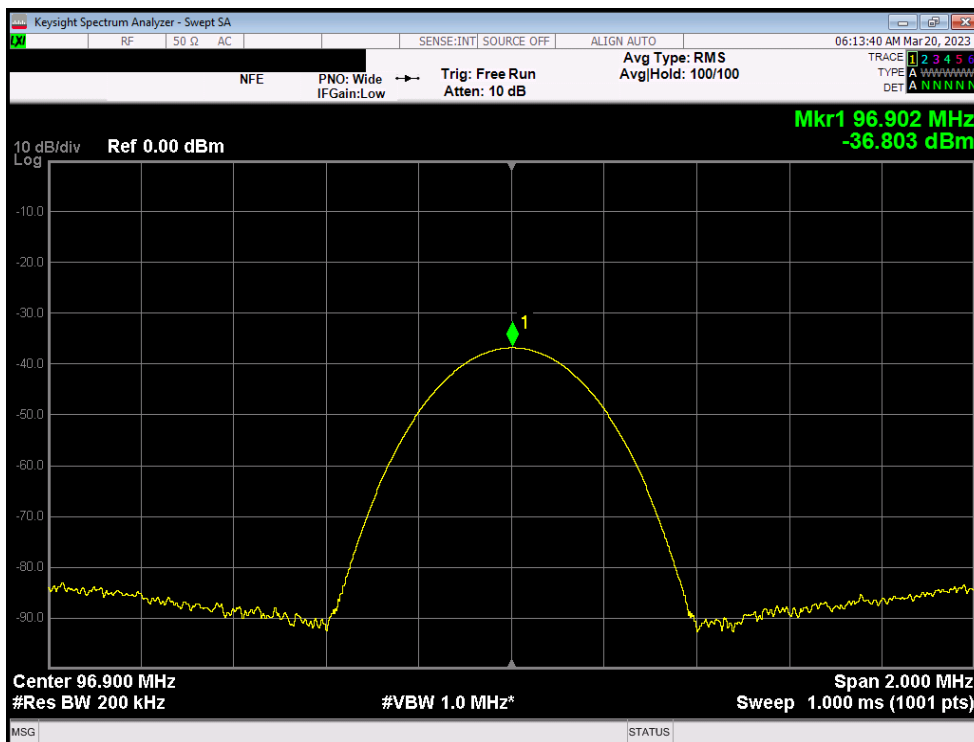
Plot 8-8. Peak Conducted Power (Channel – 96.9MHz)
