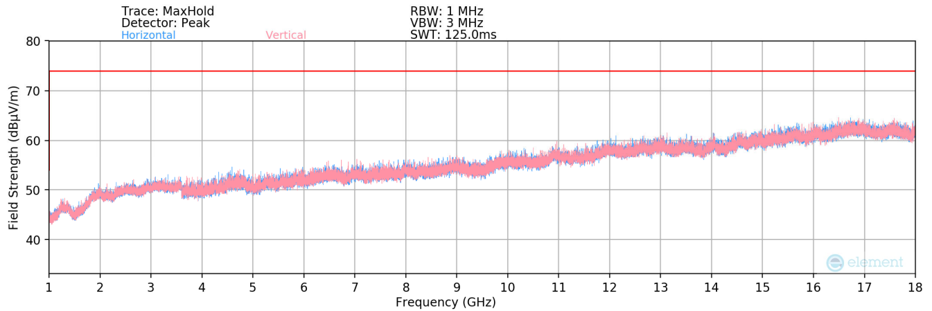
Plot 8-25. Radiated Spurious Plot above 1GHz (88.1)
