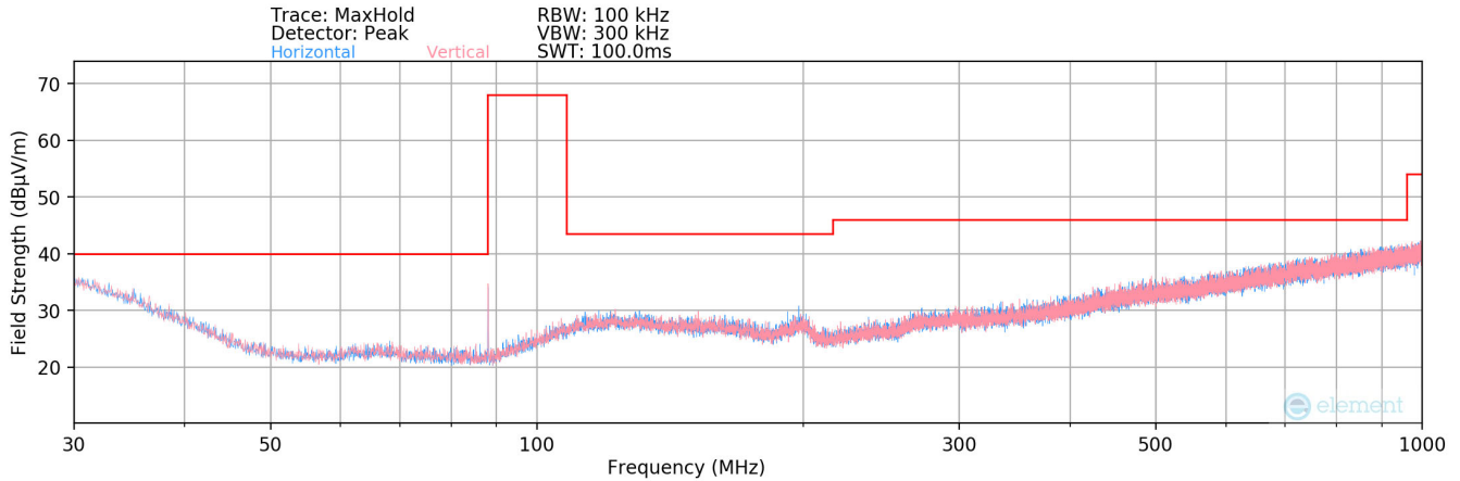
Plot 8-10. Radiated Spurious Plot below 1GHz (88.1MHz Configuration #7)
