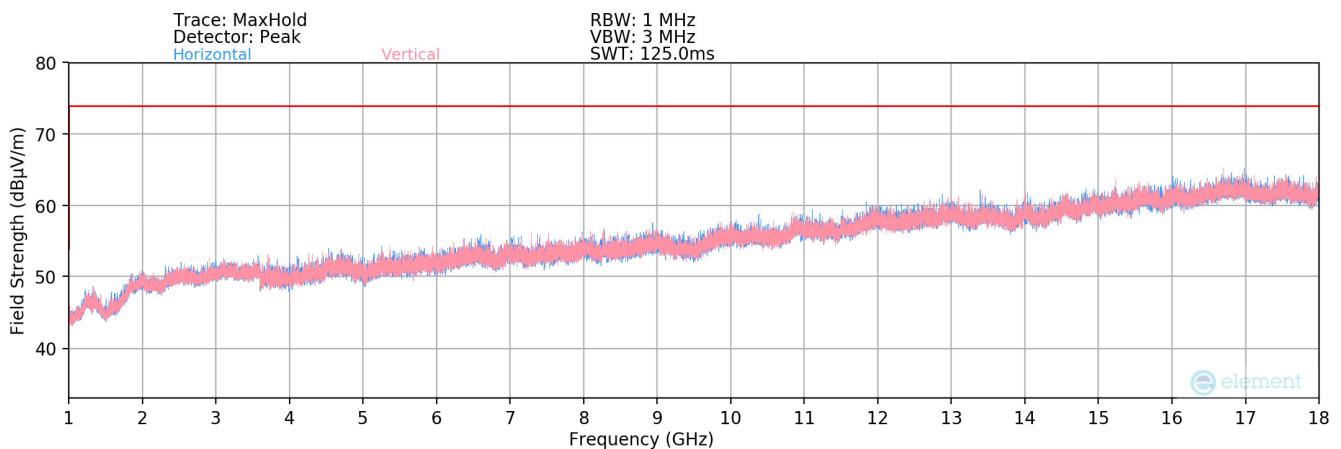
Plot 8-24. Radiated Spurious Plot above 1GHz (107.9)
