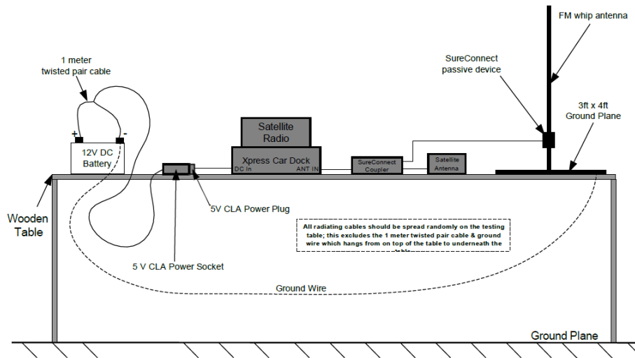
Figure 8-7. Test Instrument & Measurement Setup (Configuration #9 Xpress Car Dock & SureConnect Adapter)
