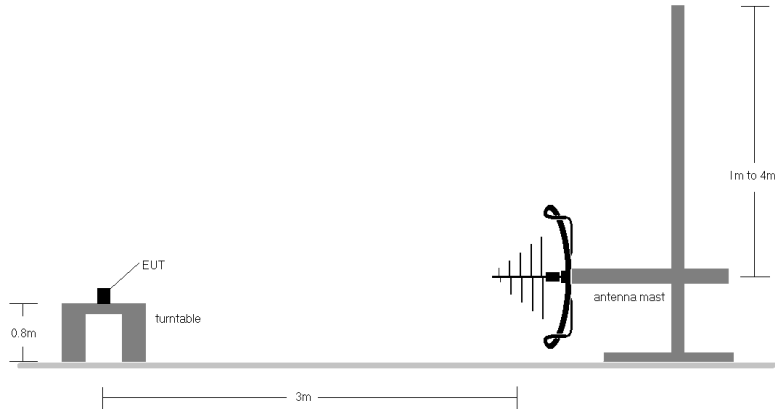
Figure 8-4. Test Instrument & Measurement Setup
