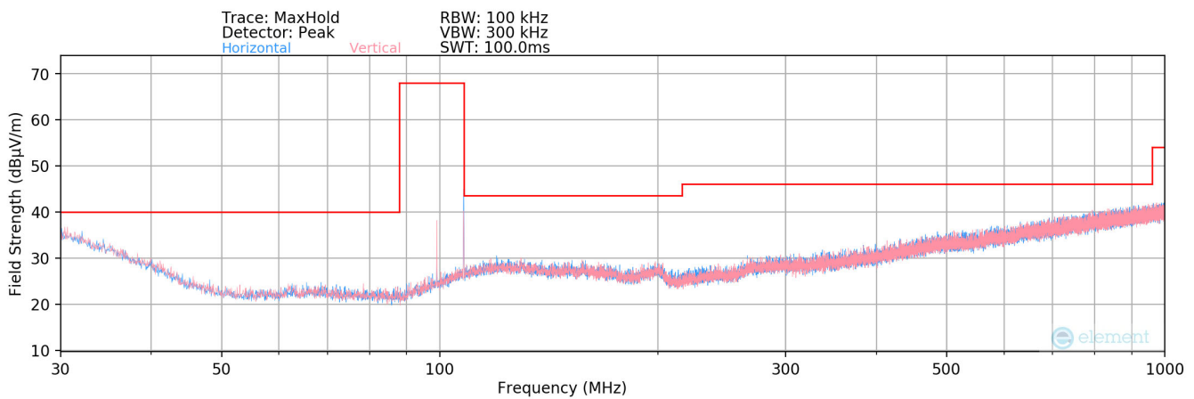
Plot 8-18. Radiated Spurious Plot below 1GHz (107.9MHz Configuration #9)
