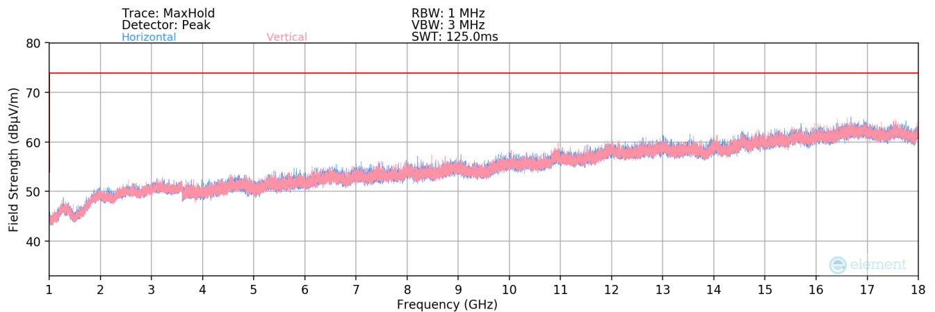
Plot 8-26. Radiated Spurious Plot above 1GHz (96.9)
