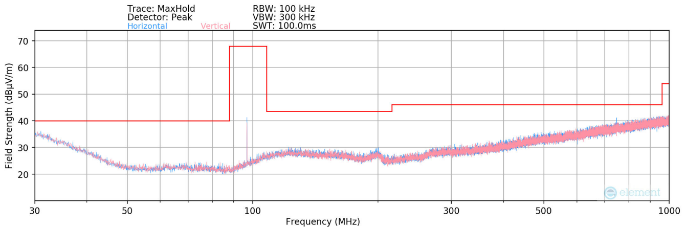
Plot 8-11. Radiated Spurious Plot below 1GHz (96.9MHz Configuration #7)
