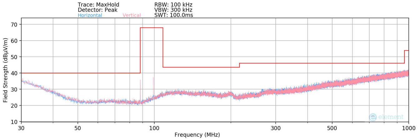
Plot 8-13. Radiated Spurious Plot below 1GHz (88.1MHz Configuration #8)
