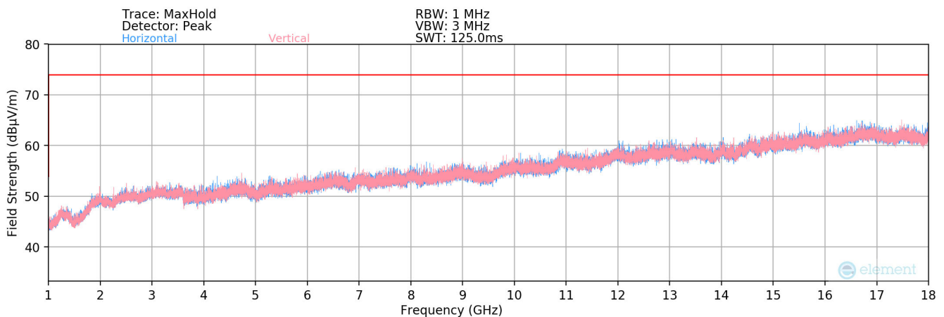
Plot 8-21. Radiated Spurious Plot above 1GHz (107.9MHz)
