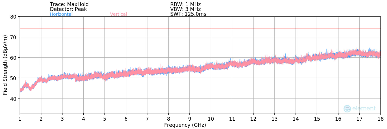
Plot 8-22. Radiated Spurious Plot above 1GHz (88.1)
