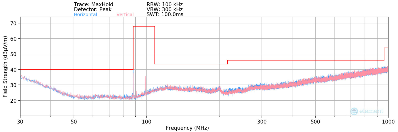
Plot 8-16. Radiated Spurious Plot below 1GHz (88.1MHz Configuration #9)
