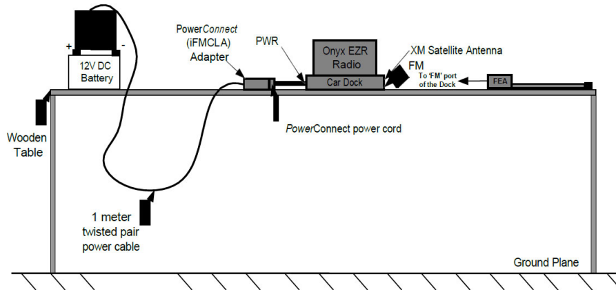
Figure 8-5. Test Instrument & Measurement Setup (Configuration #7 FEA unit)
