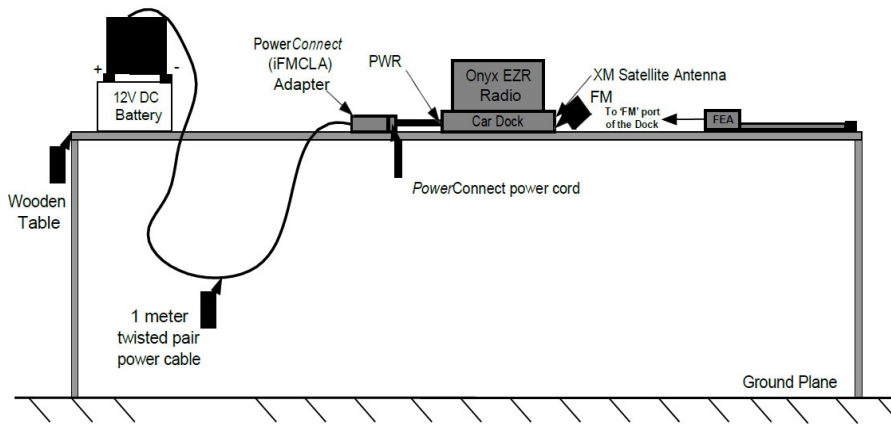
Figure 8-9. Test Instrument & Measurement Setup (Configuration #7 FEA unit)
