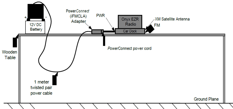
Figure 8-6. Test Instrument & Measurement Setup (Configuration #8 PowerConnect only)
