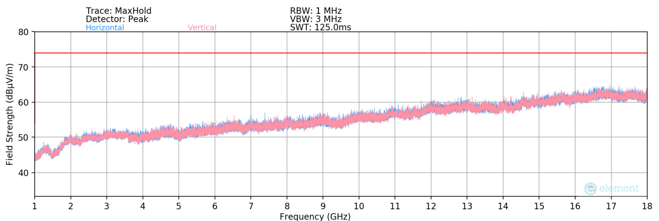
Plot 8-27. Radiated Spurious Plot above 1GHz (107.9)
