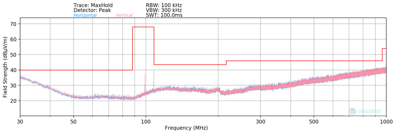
Plot 8-15. Radiated Spurious Plot below 1GHz (107.9MHz Configuration #8)
