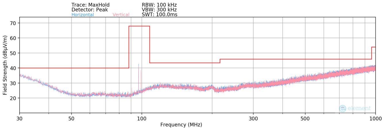
Plot 8-17. Radiated Spurious Plot below 1GHz (96.9MHz Configuration #9)
