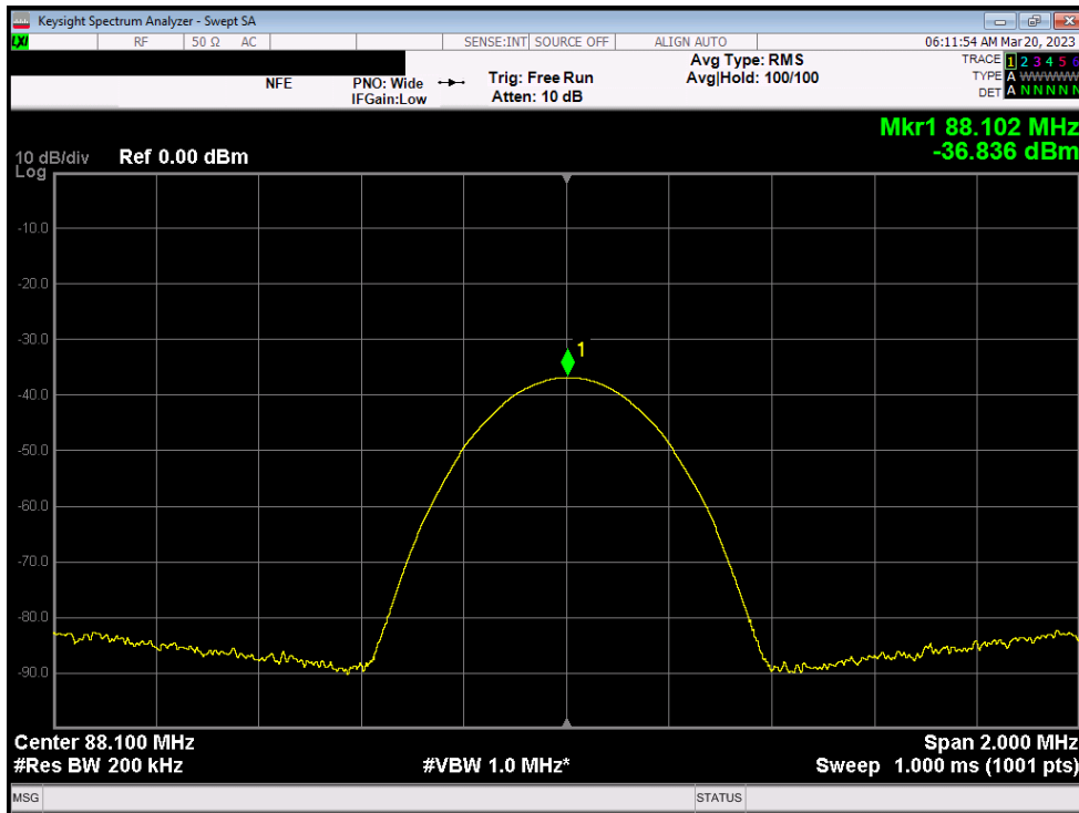
Plot 8-7. Peak Conducted Power (Low Channel – 88.1MHz)
