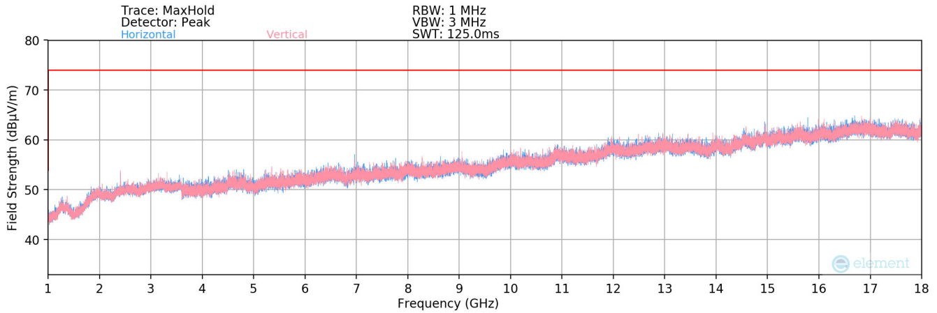
Plot 8-19. Radiated Spurious Plot above 1GHz (88.1MHz)
