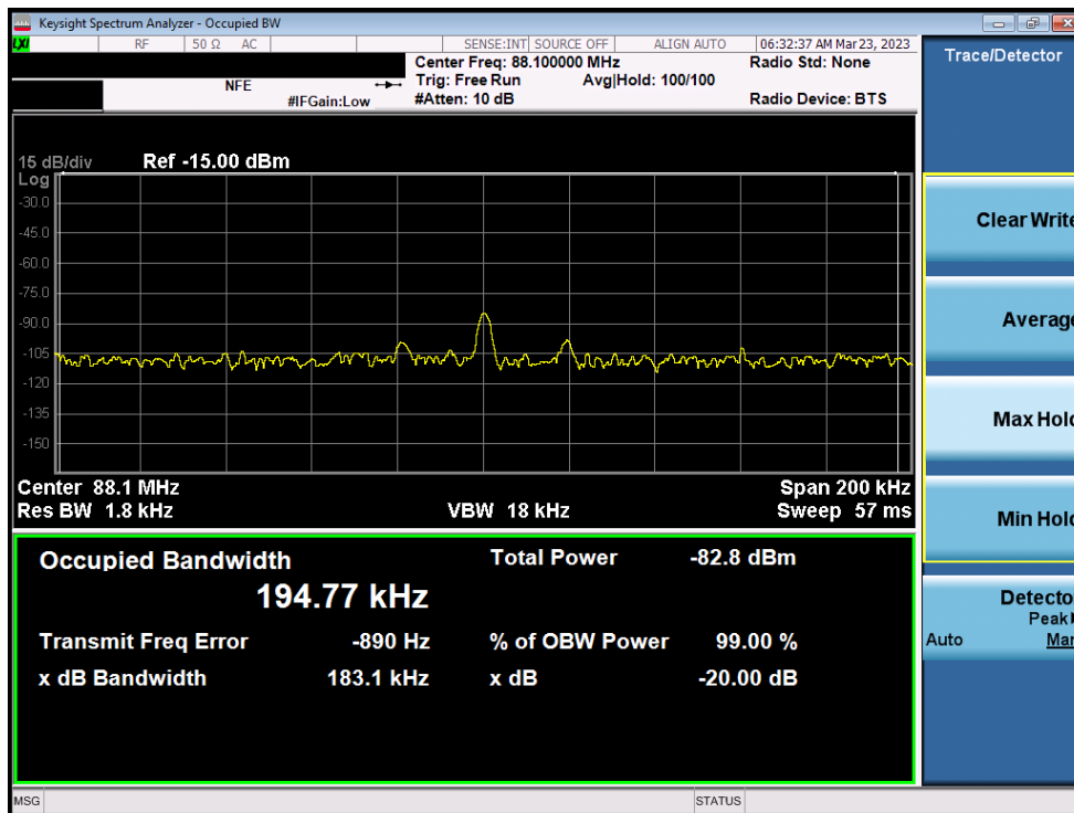
Plot 8-4. 20dB Bandwidth Plot (Low Channel – 88.1MHz)
