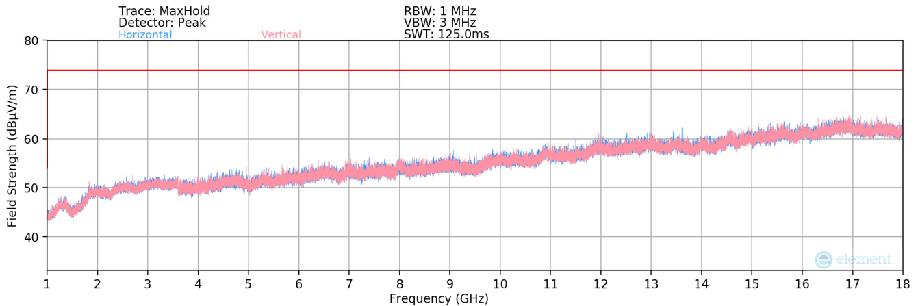
Plot 8-23. Radiated Spurious Plot above 1GHz (96.9)
