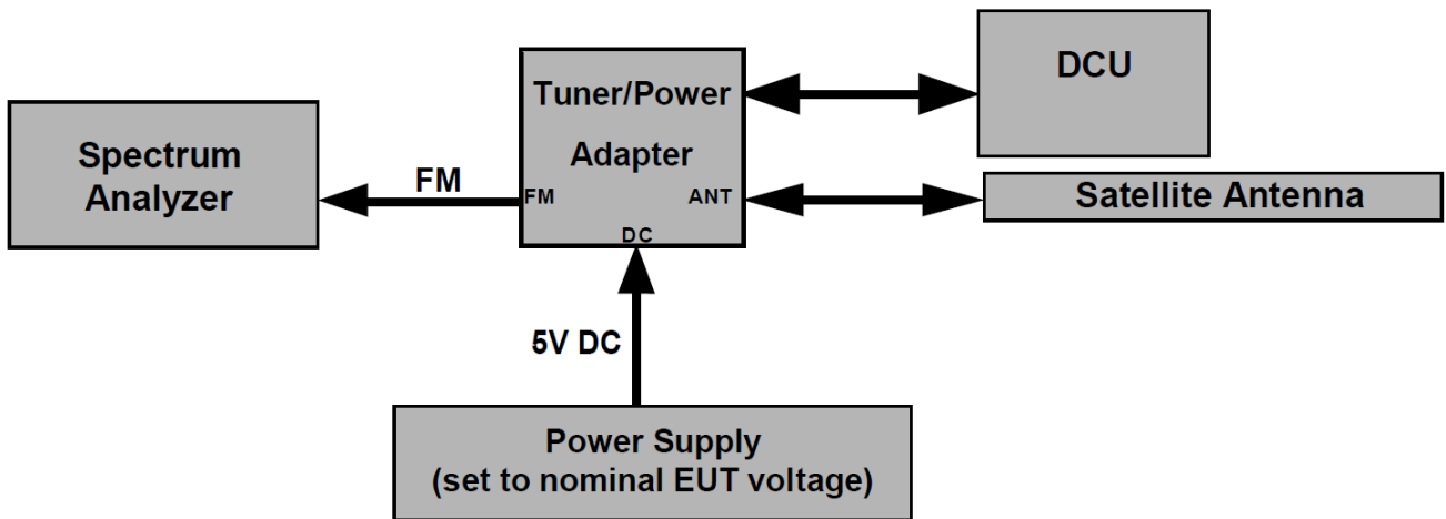
Figure 8-1. Test Instrument & Measurement Setup (Configuration #5 PowerConnect Car Dock & iFMCLA)
