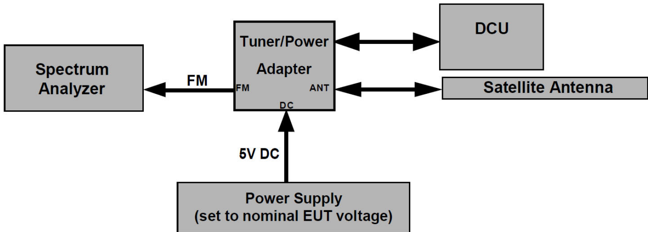
Figure 8-3. Test Instrument & Measurement Setup (Configuration #10)
