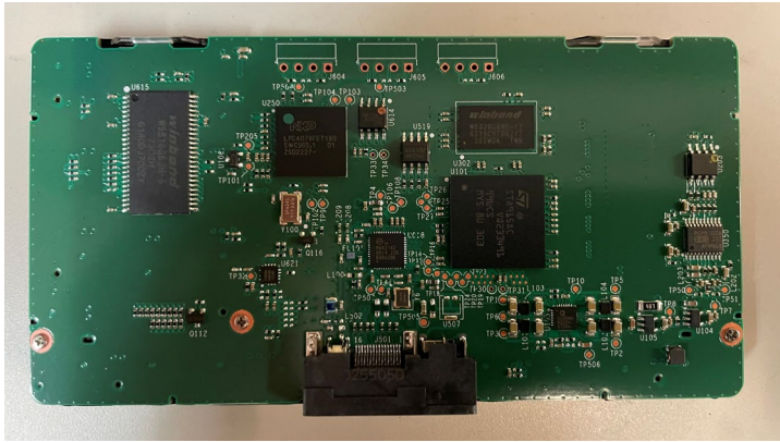
PCBA Rear View (w/front housing & screws)
