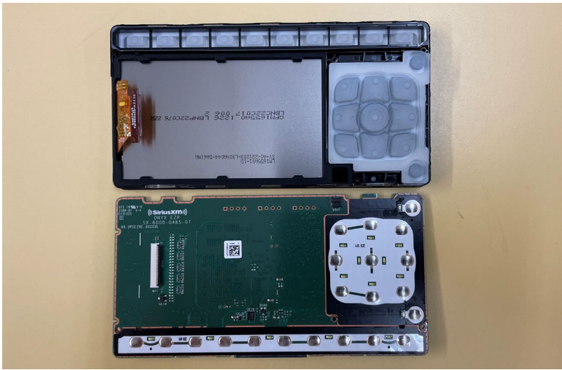
Front View with Front Housing, Keypad(s) and Display Removed
