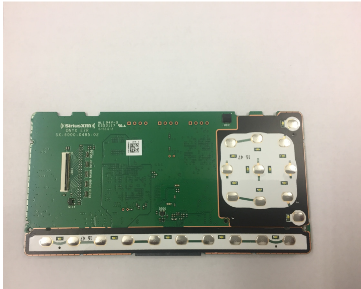
PCBA Front View (w/popple domes)
