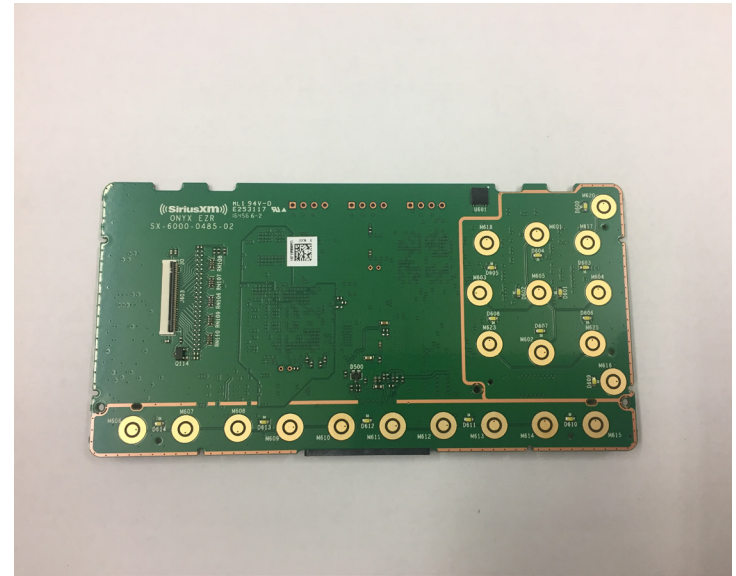
PCBA Front View (no popple domes)
