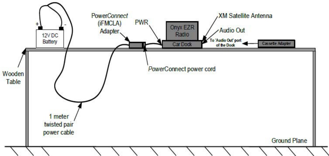
Figure 7-5. Test Instrument & Measurement Setup (Configuration #4)
