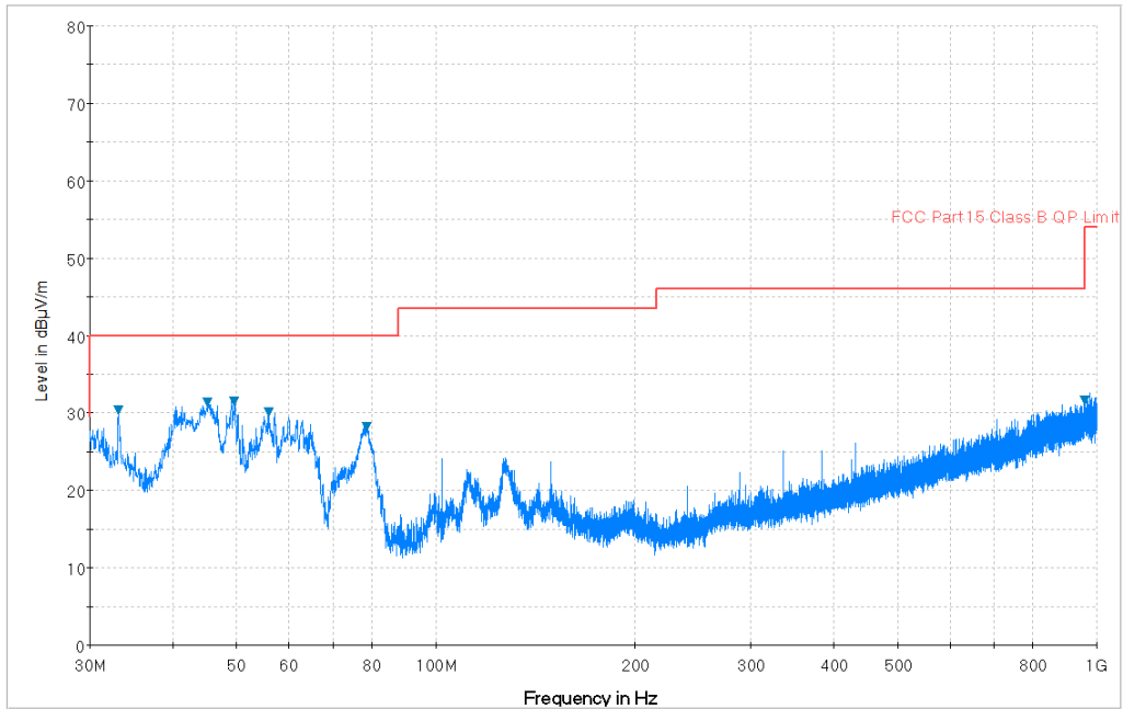
Plot 7-2. Radiated Spurious Plot below 1GHz (Configuration #2, Pol. V)
