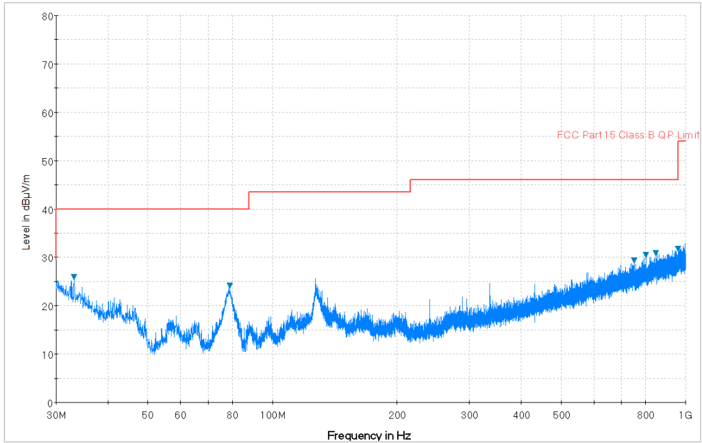
Plot 7-1. Radiated Spurious Plot below 1GHz (Configuration #2, Pol. H)
