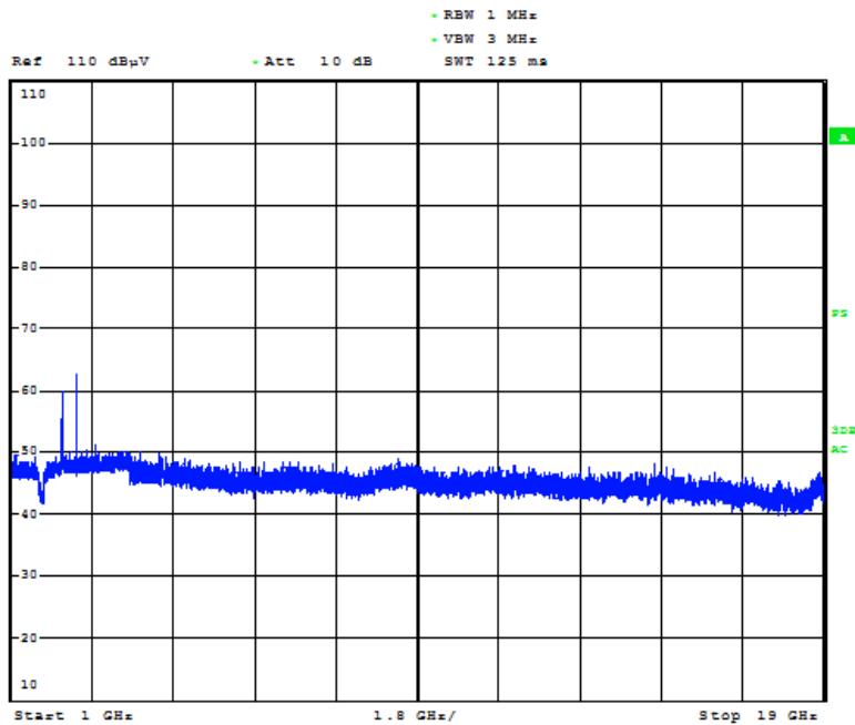
Plot 7-7. Radiated Spurious Plot above 1GHz (Configuration #3, Pol. H)
