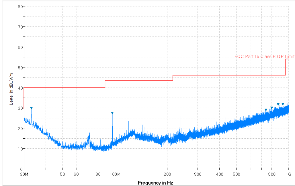
Plot 7-5. Radiated Spurious Plot below 1GHz (Configuration #3, Pol. H)
