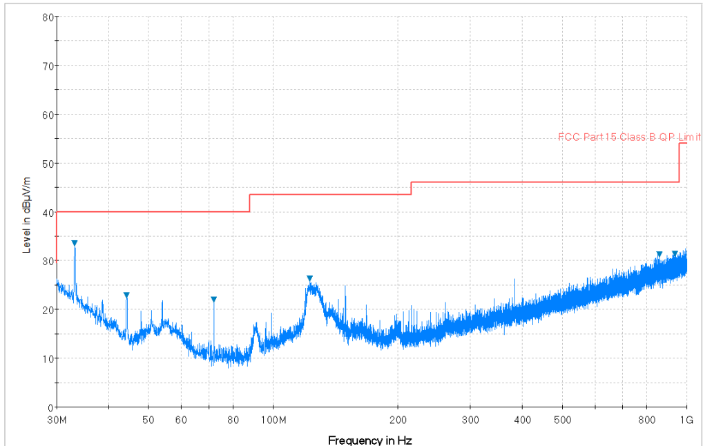
Plot 7-10. Radiated Spurious Plot below 1GHz (Configuration #4, Pol. V)
