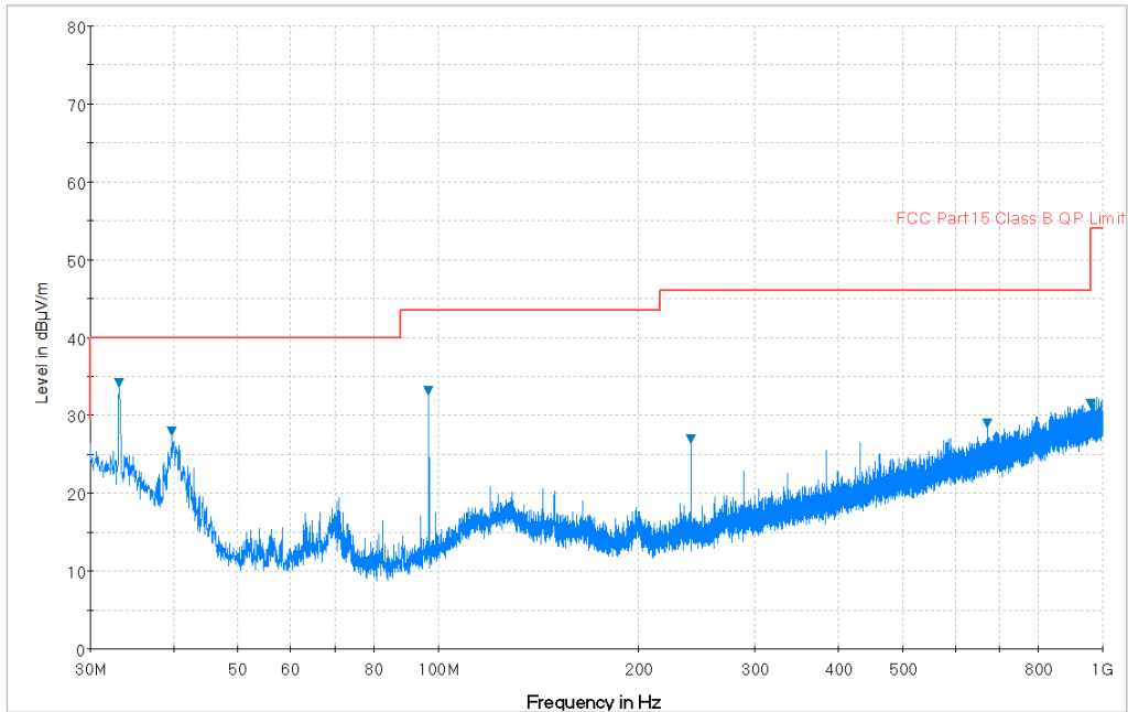
Plot 7-6. Radiated Spurious Plot below 1GHz (Configuration #3, Pol. V)
