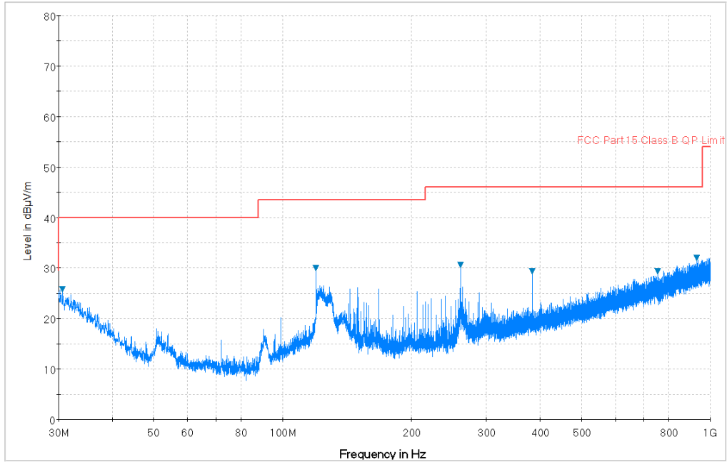
Plot 7-9. Radiated Spurious Plot below 1GHz (Configuration #4, Pol. H)
