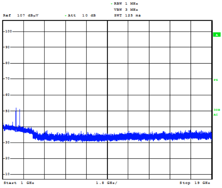
Plot 7-3. Radiated Spurious Plot above 1GHz (Configuration #2, Pol. H)
