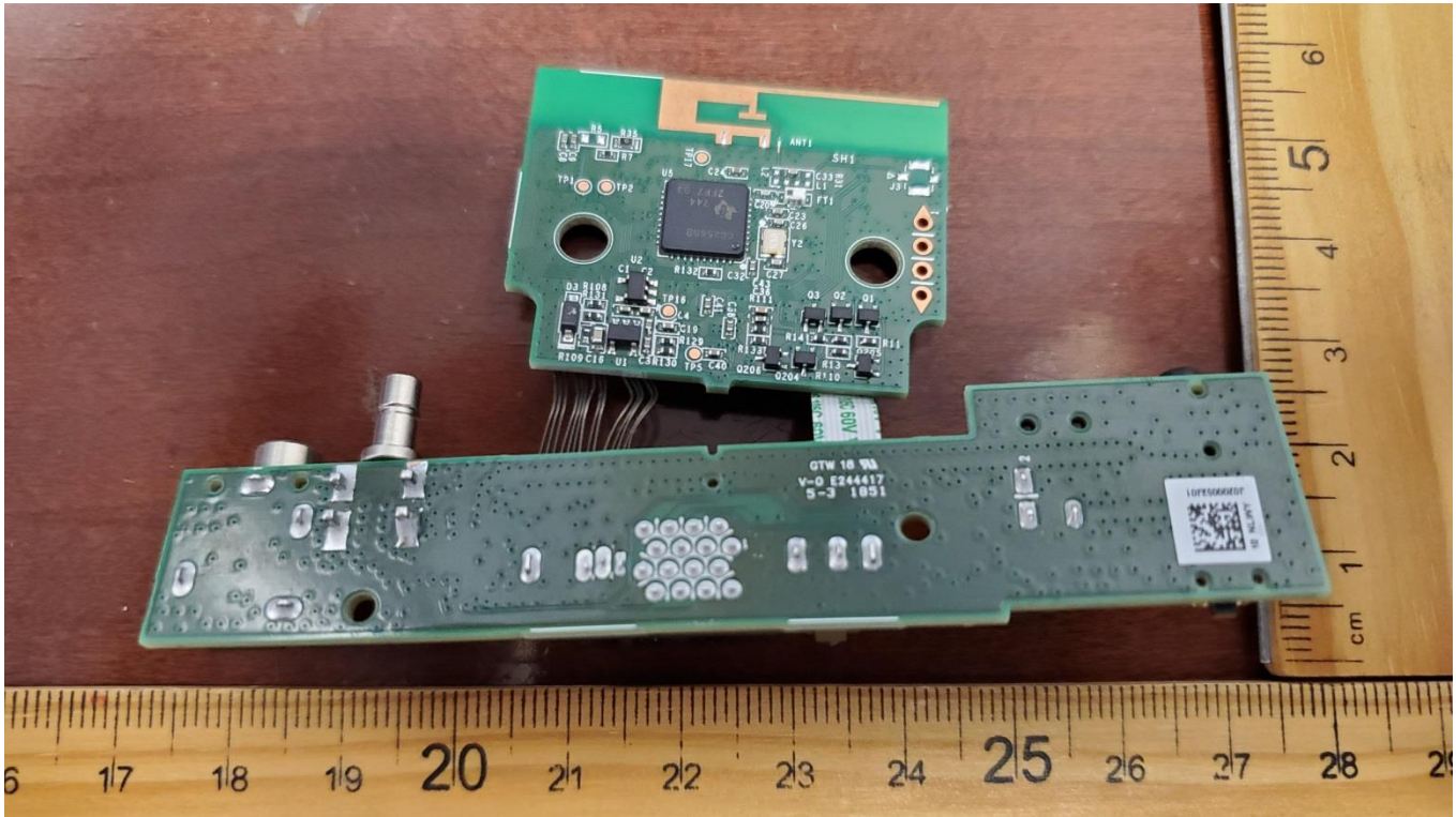
Figure 2: Bottom Side
