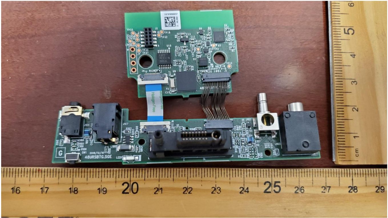
Figure 1: Top side
