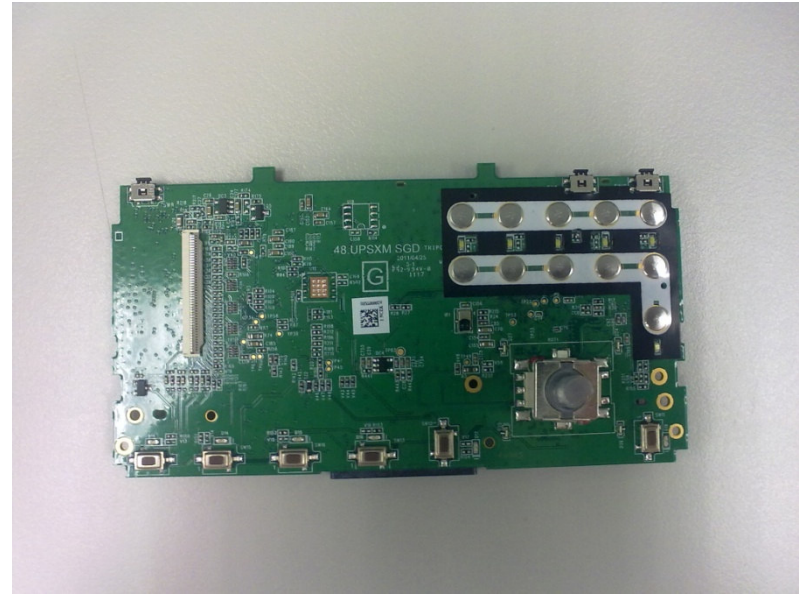
PCBA front without LCM (with front housing removed)
