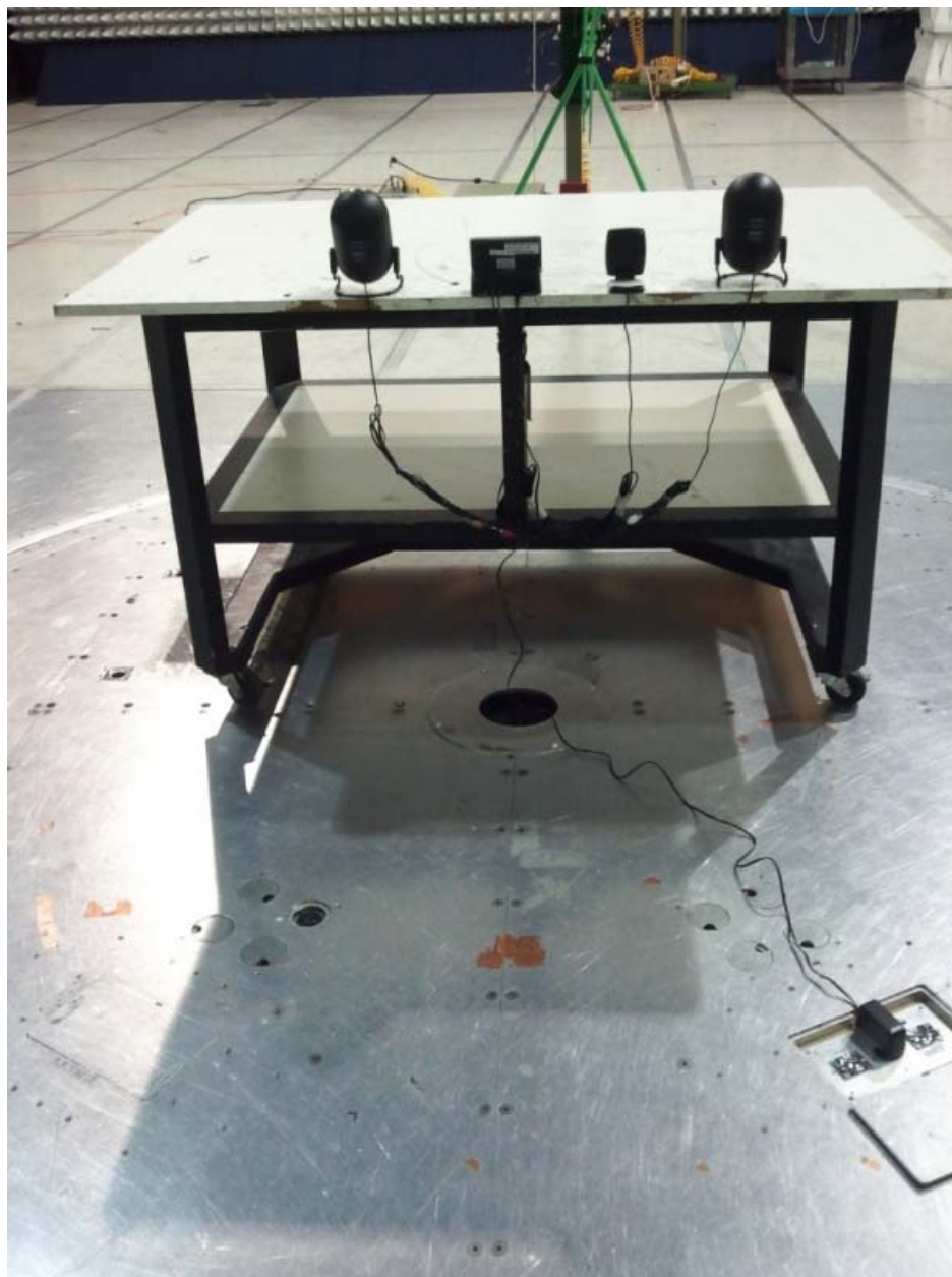
HomeDock Radiated Emissions Test Setup - Rear View
