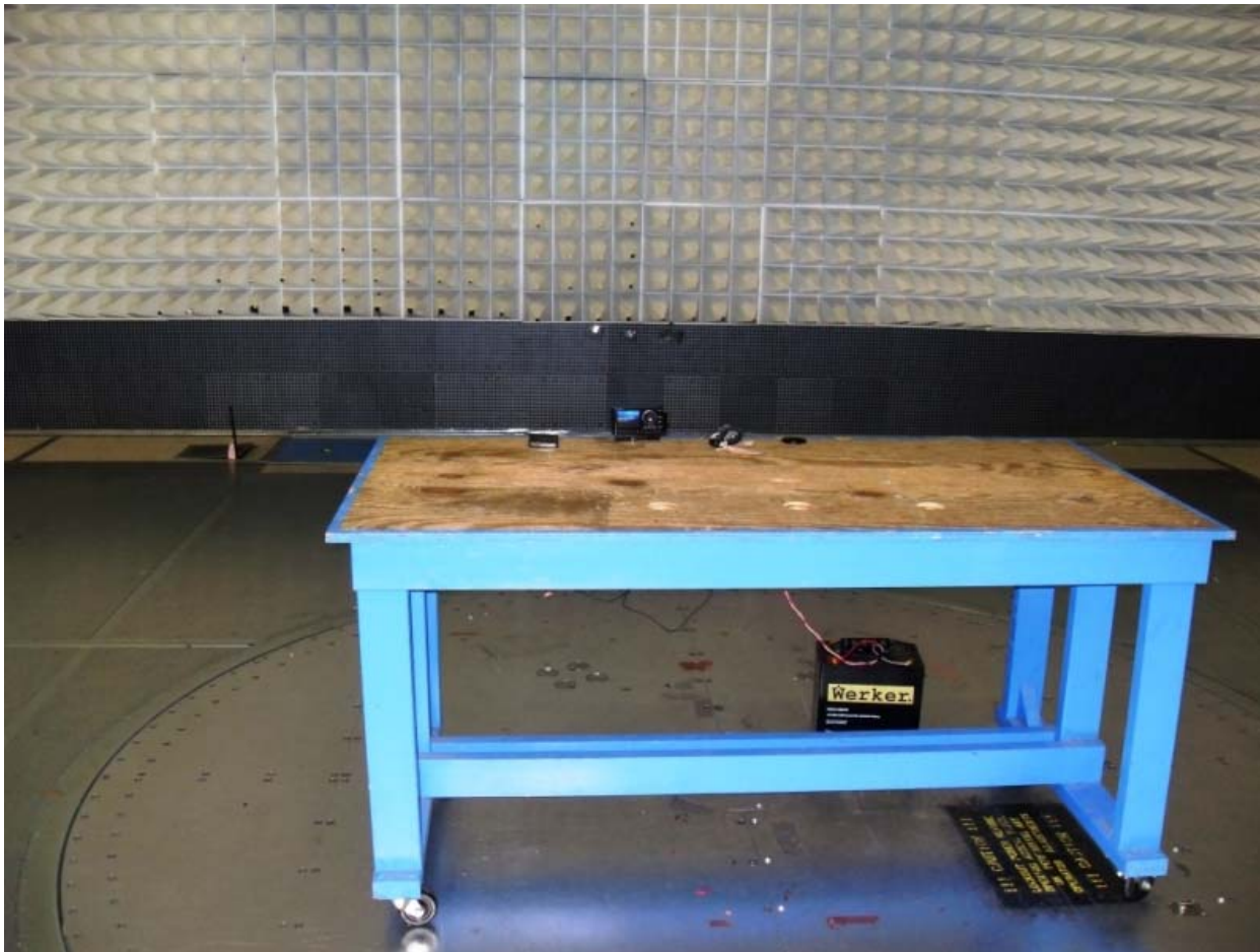
Cassette Adapter Test Setup - Front View
