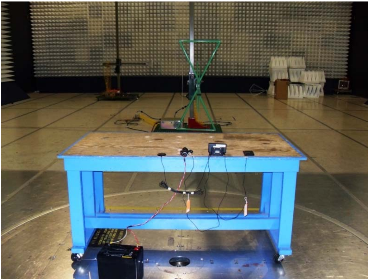
Cassette Adapter Test Setup - Rear View
