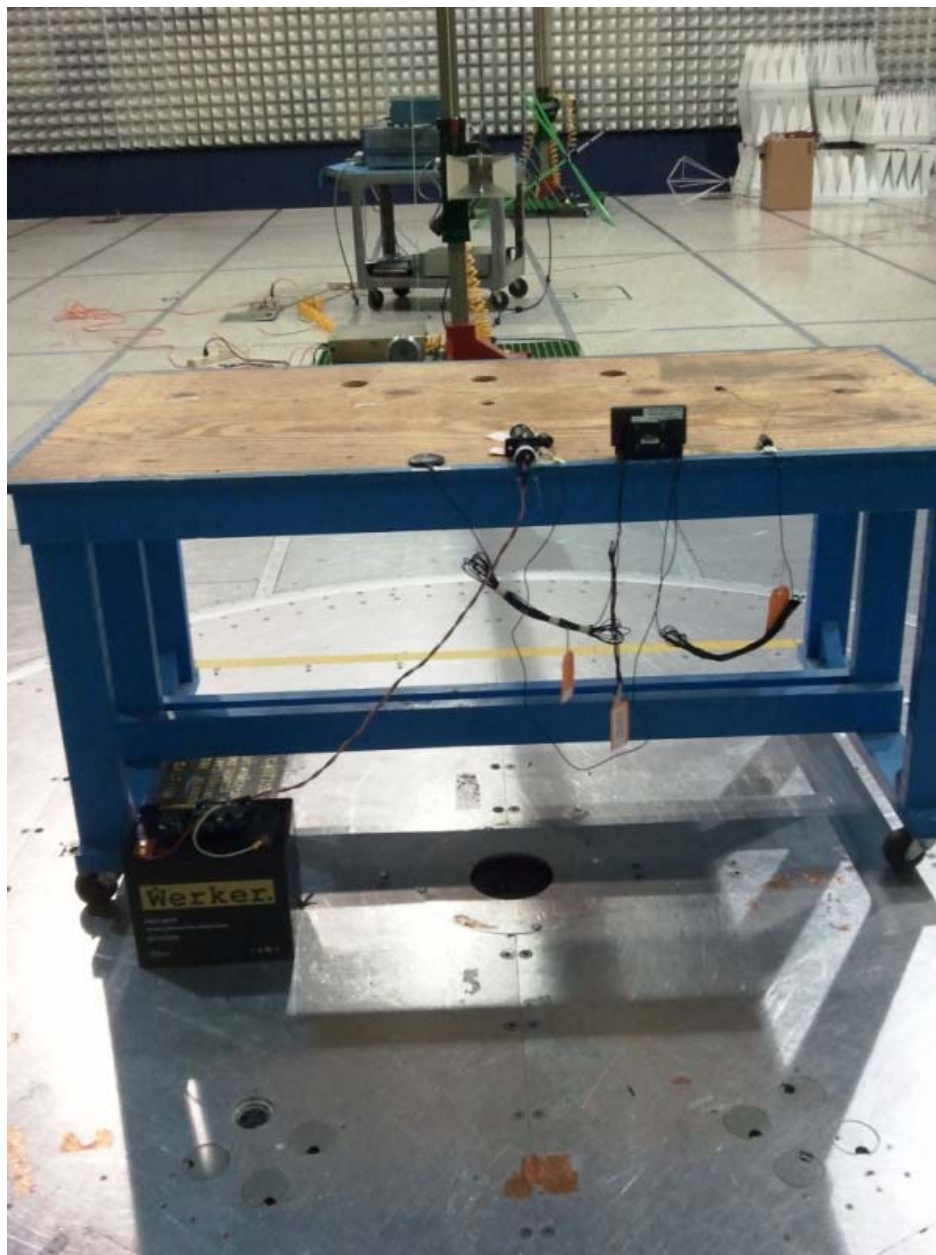
FEA Adapter Test Setup - Rear View
