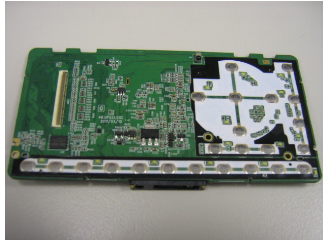
Front View of PCB without LCM
