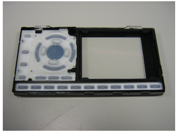
Front View (with Front Housing Removed)
