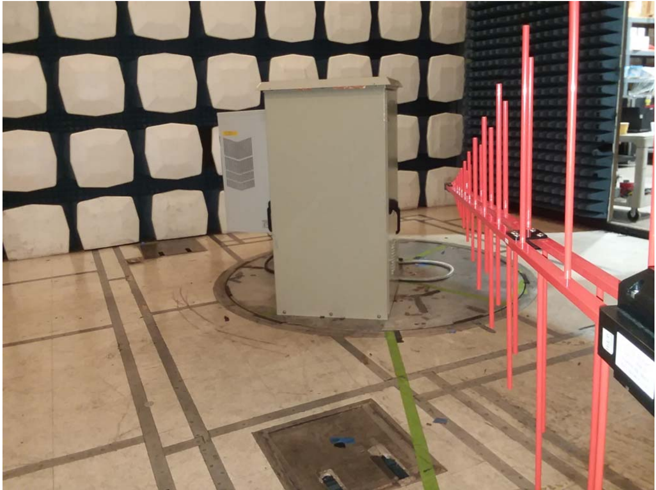
Photograph 2. Cabinet Spurious Radiation, Test Setup 1
