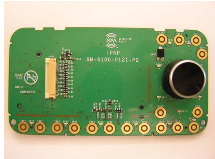
XM PCBA Front View (no popple domes)
