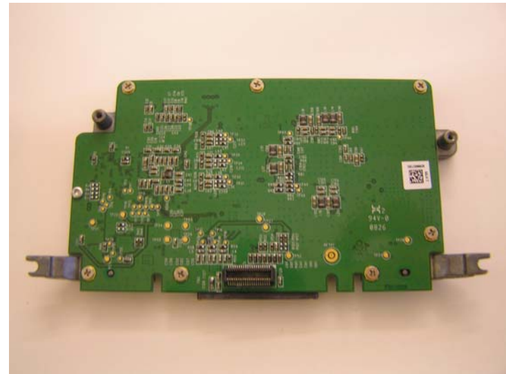
Sirius (Picasso) PCBA Front View (w/heat sink)
