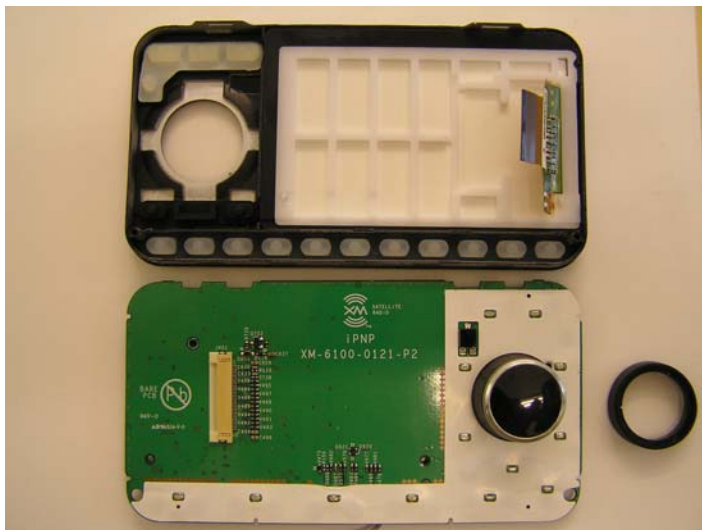
iPNP Front View with Front Housing, Keypad(s) and display
