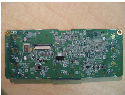
Front View PCBA (without LCD/Frame)
