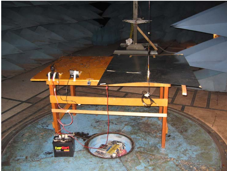
RodyXT with Aerial Antenna Coupler, View 1
