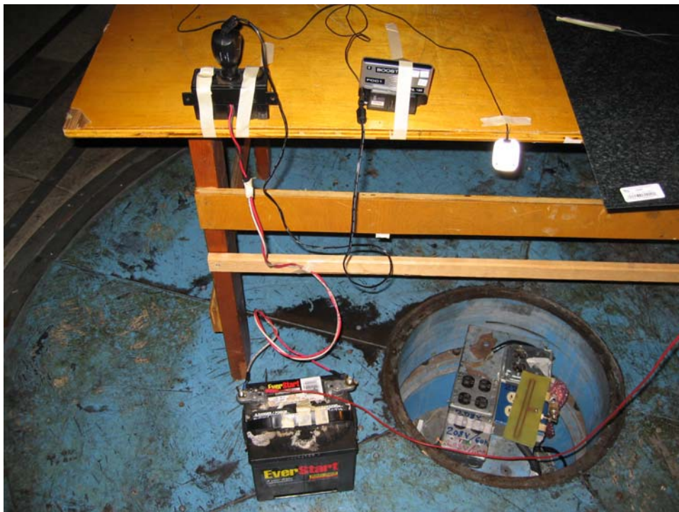
RodyXT with Aerial Antenna Coupler, View 2
