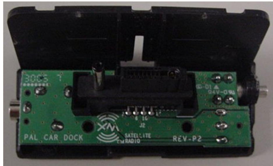
Case Open with PCB Inside
