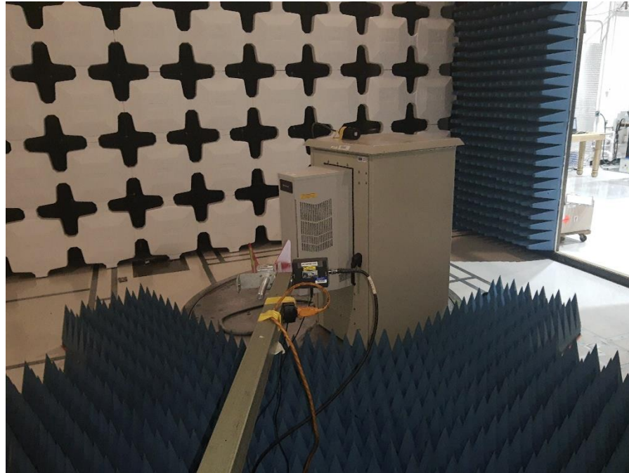
Cabinet Spurious Emissions, Test Setup Above 1 GHz
