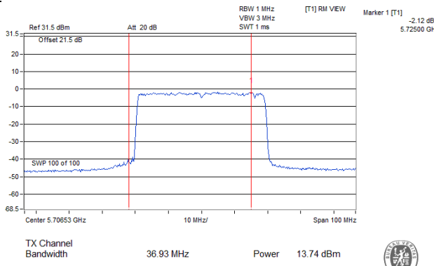
802.11ax (HE40)_Chain 3 / CH142 (U-NII-2C Band)
