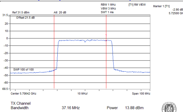
802.11ax (HE40)_Chain 1 / CH142 (U-NII-2C Band)
