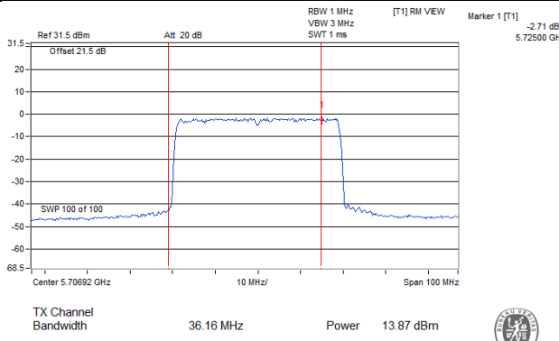
802.11ax (HE40)_Chain 2 / CH142 (U-NII-2C Band)
