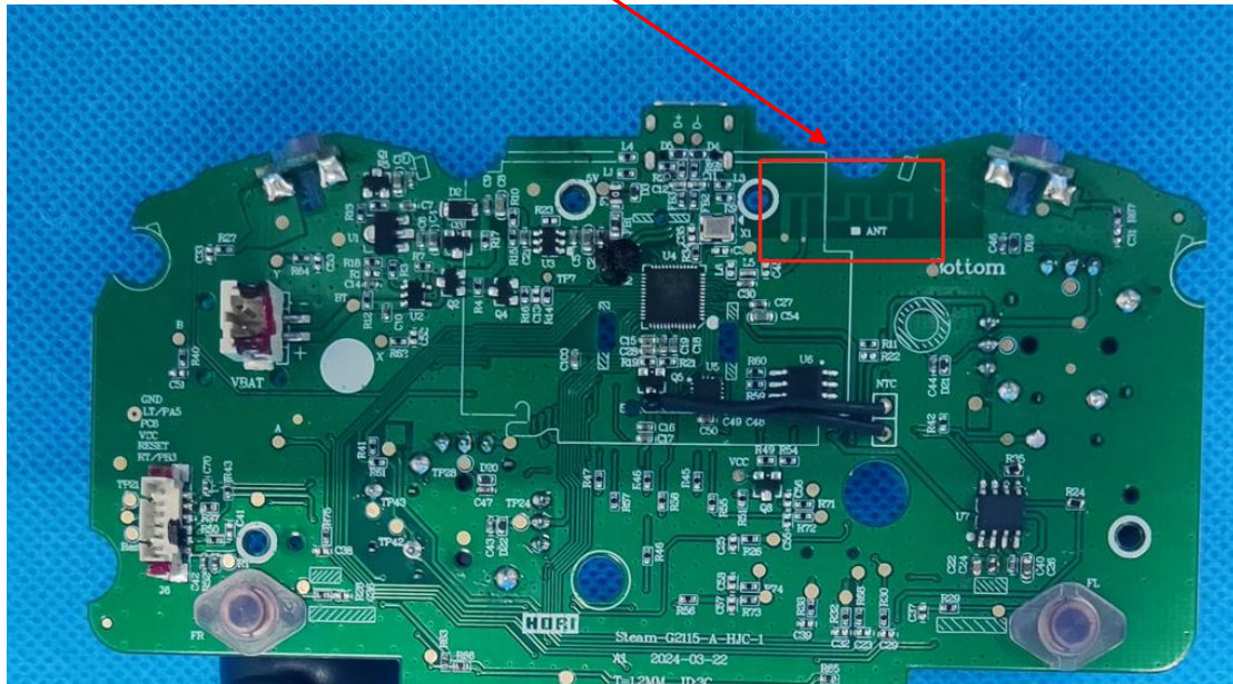
View of BT antenna
