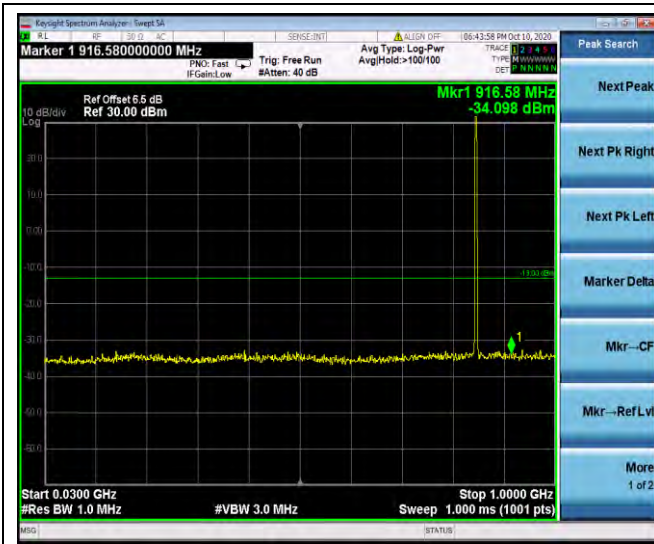
30MHz~1GHz
