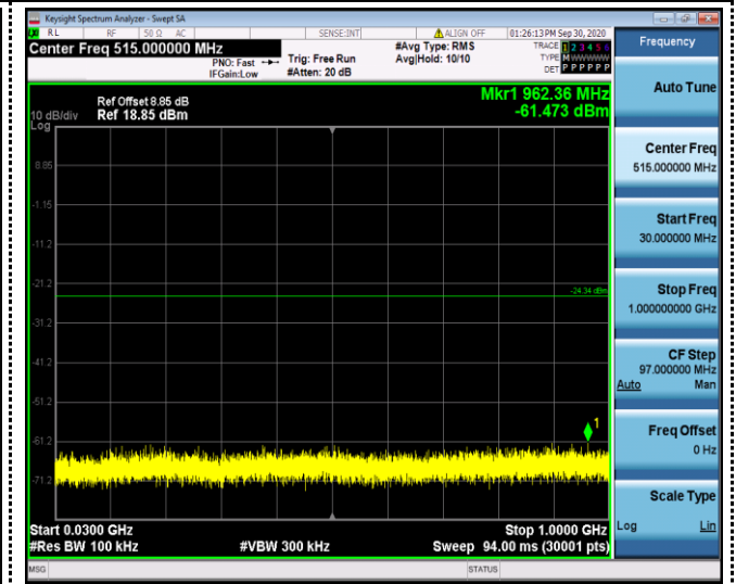
30MHz-1GHz
