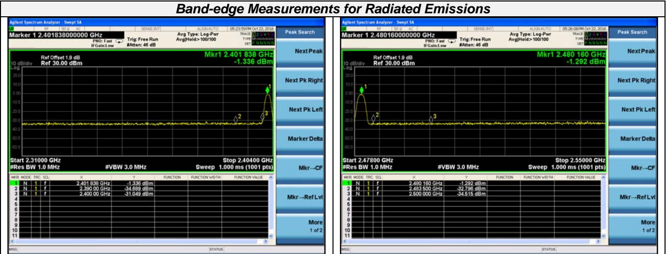
Channel 0 / 2402 MHz – Peak
