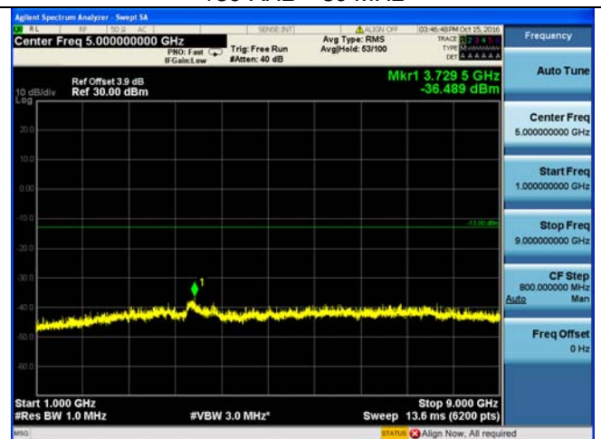
1 GHz – 9 GHz
