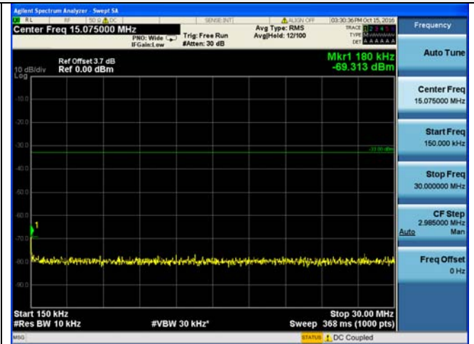
150 KHz – 30 MHz
