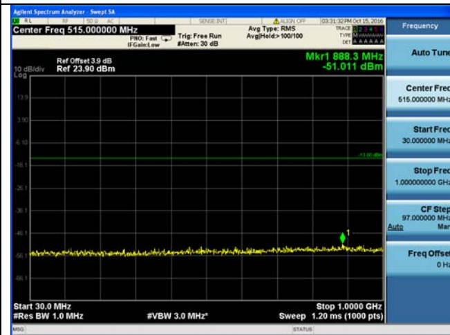
30 MHz – 1 GHz
