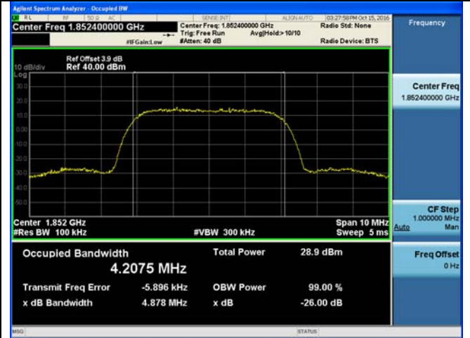
Channel 9262 / 1852.4 MHz
