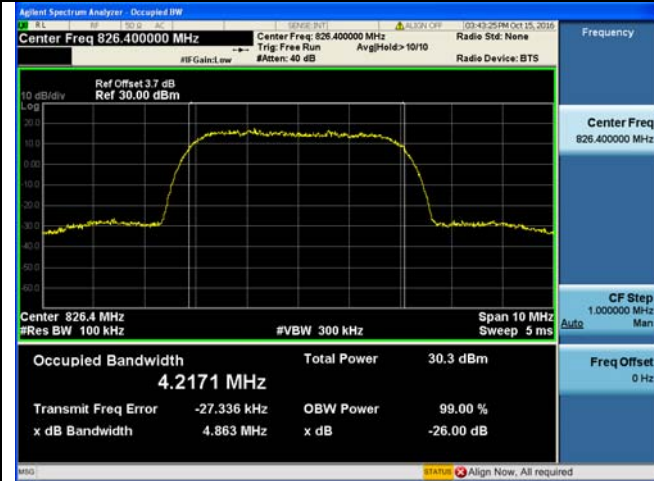
Channel 4132 / 826.4 MHz
