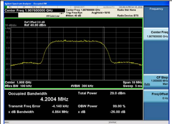
Channel 9538 / 1907.6 MHz
