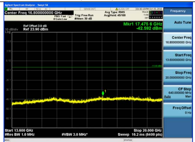
13.6 GHz – 20 GHz
