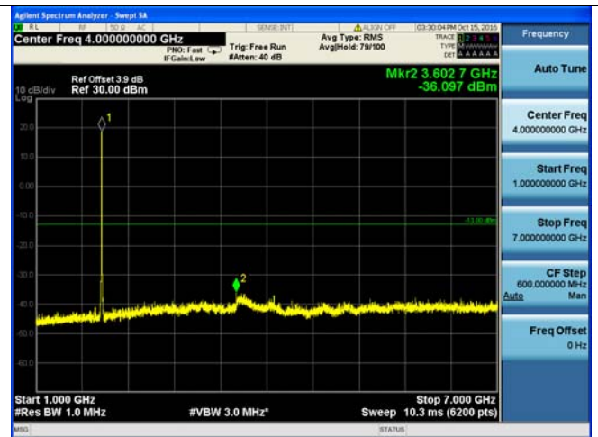
1 GHz – 7 GHz
