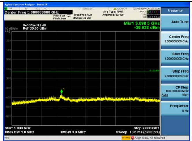
1 GHz – 9 GHz
