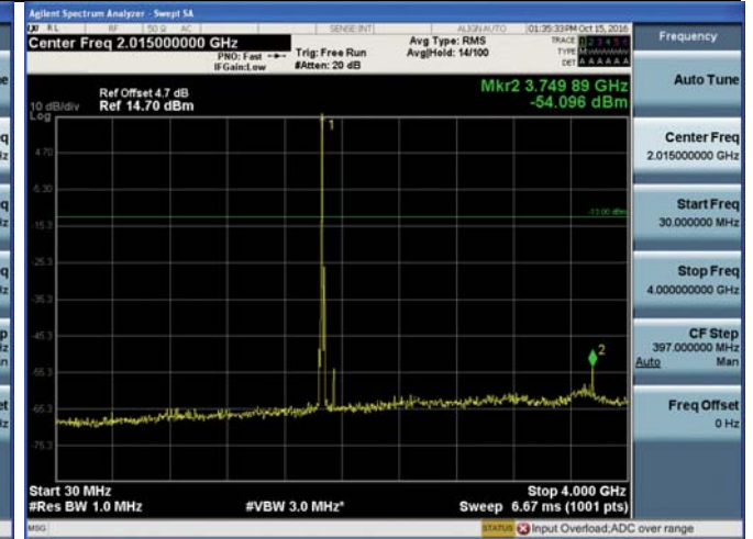
30 MHz – 4 GHz
