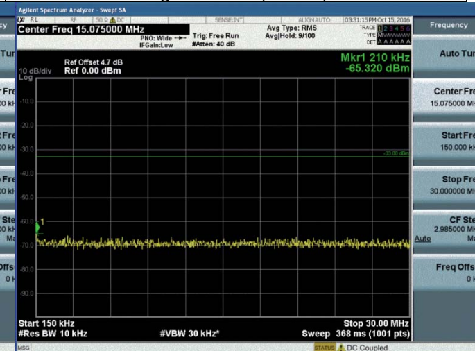
150 KHz – 30 MHz
