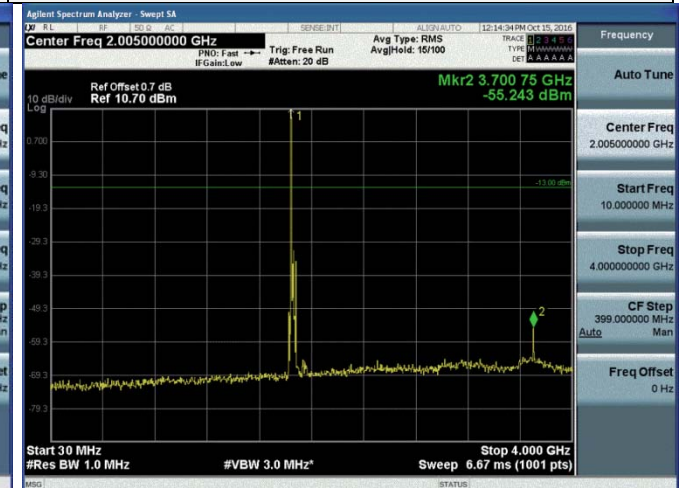
30 MHz – 4 GHz
