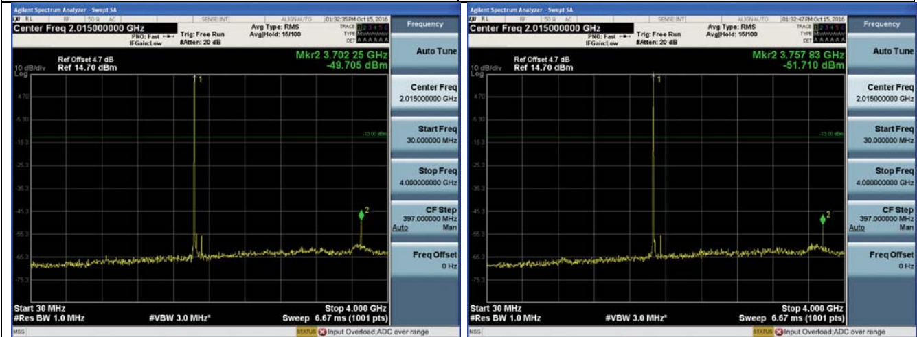
30 MHz – 4 GHz
