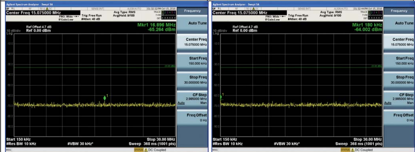
150 KHz – 30 MHz
