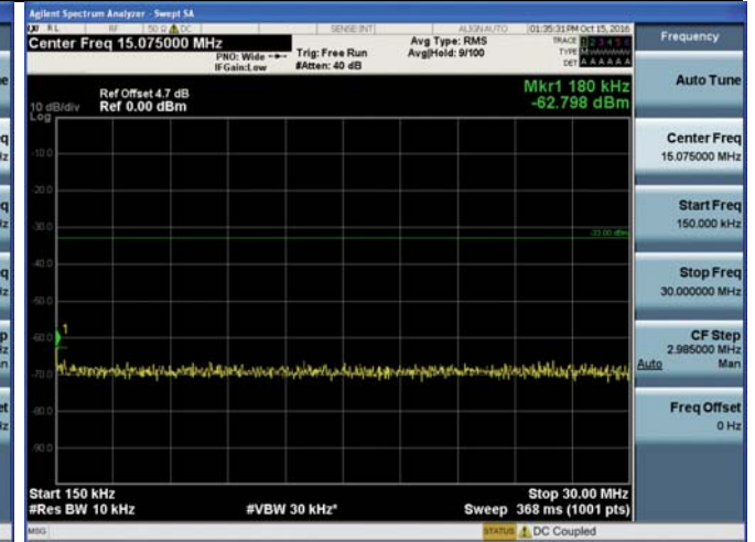
150 KHz – 30 MHz
