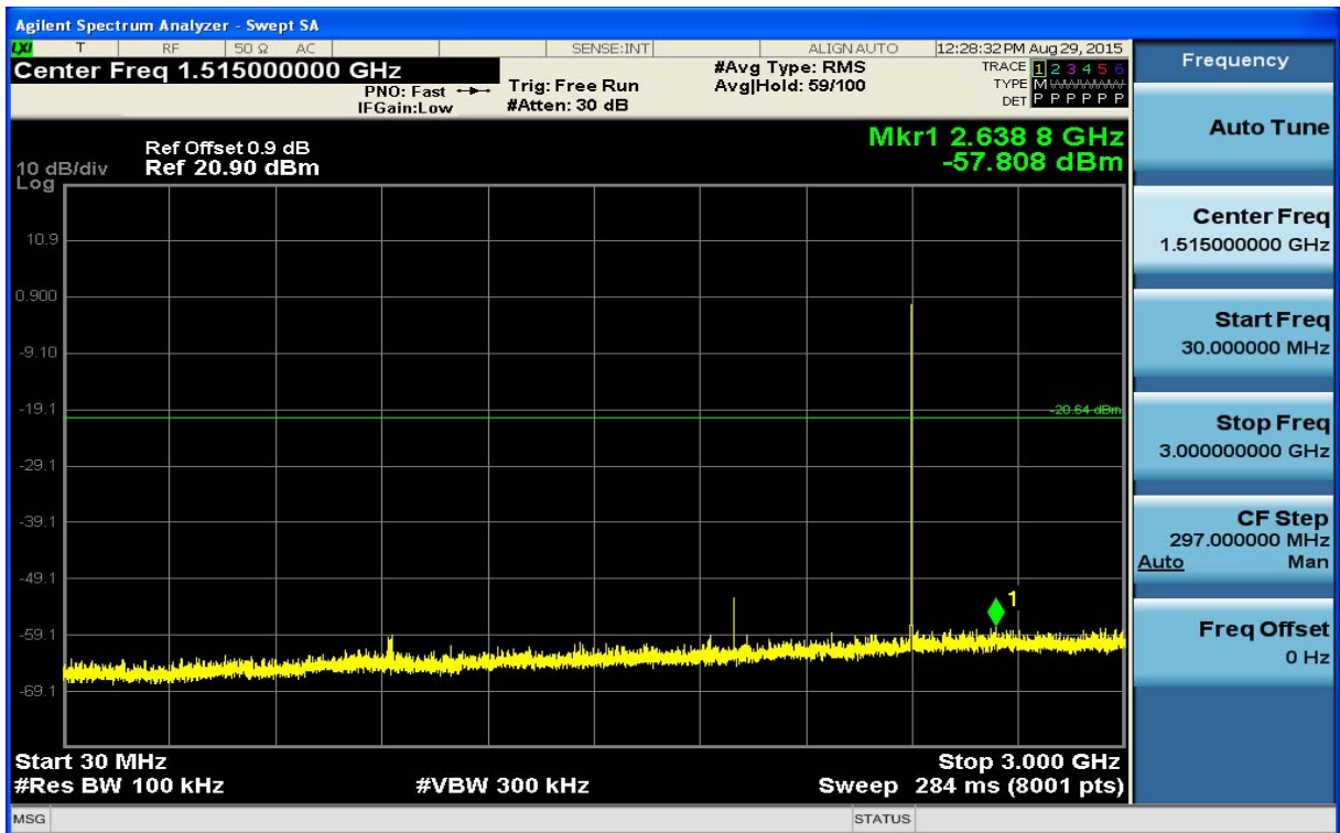
(Plot 4.6.1 A2: Channel 00: 2402MHz @ GFSK)
