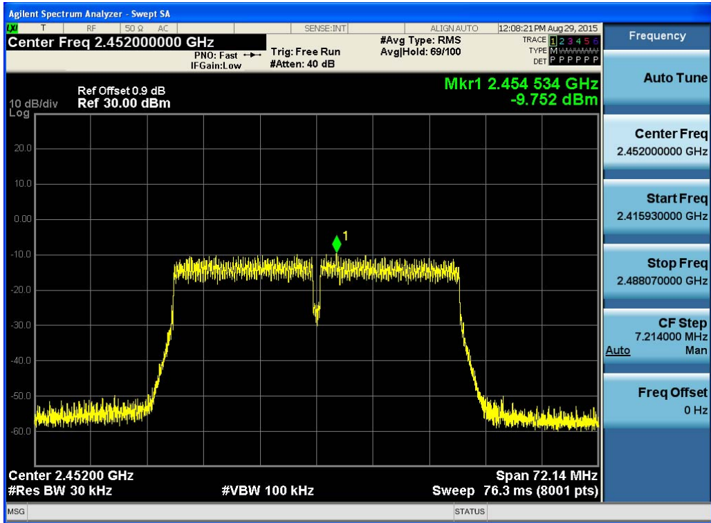
(Plot 4.4.4 C: Channel 9: 2452MHz @ 802.11n HT40)
