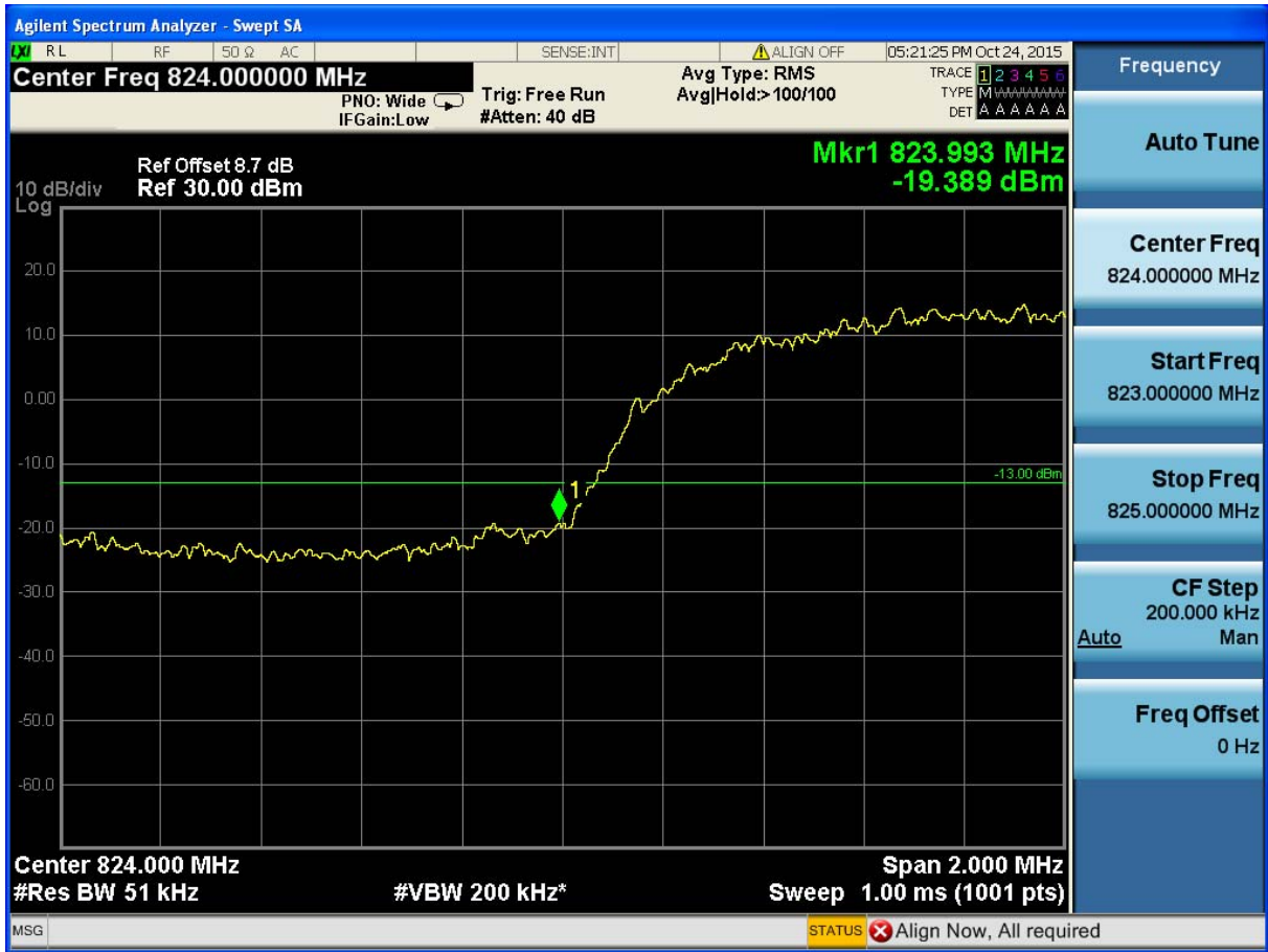
(Plot 4.5.3 A: Channel 4132: 826.4MHz @ WCDMA Band V)
