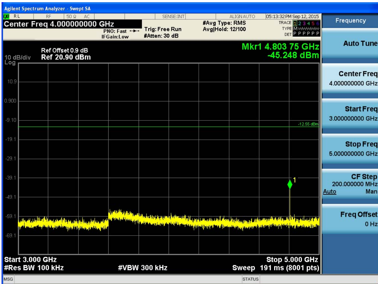
(Plot 4.6.1 A3: Channel 00: 2402MHz @ GFSK)
