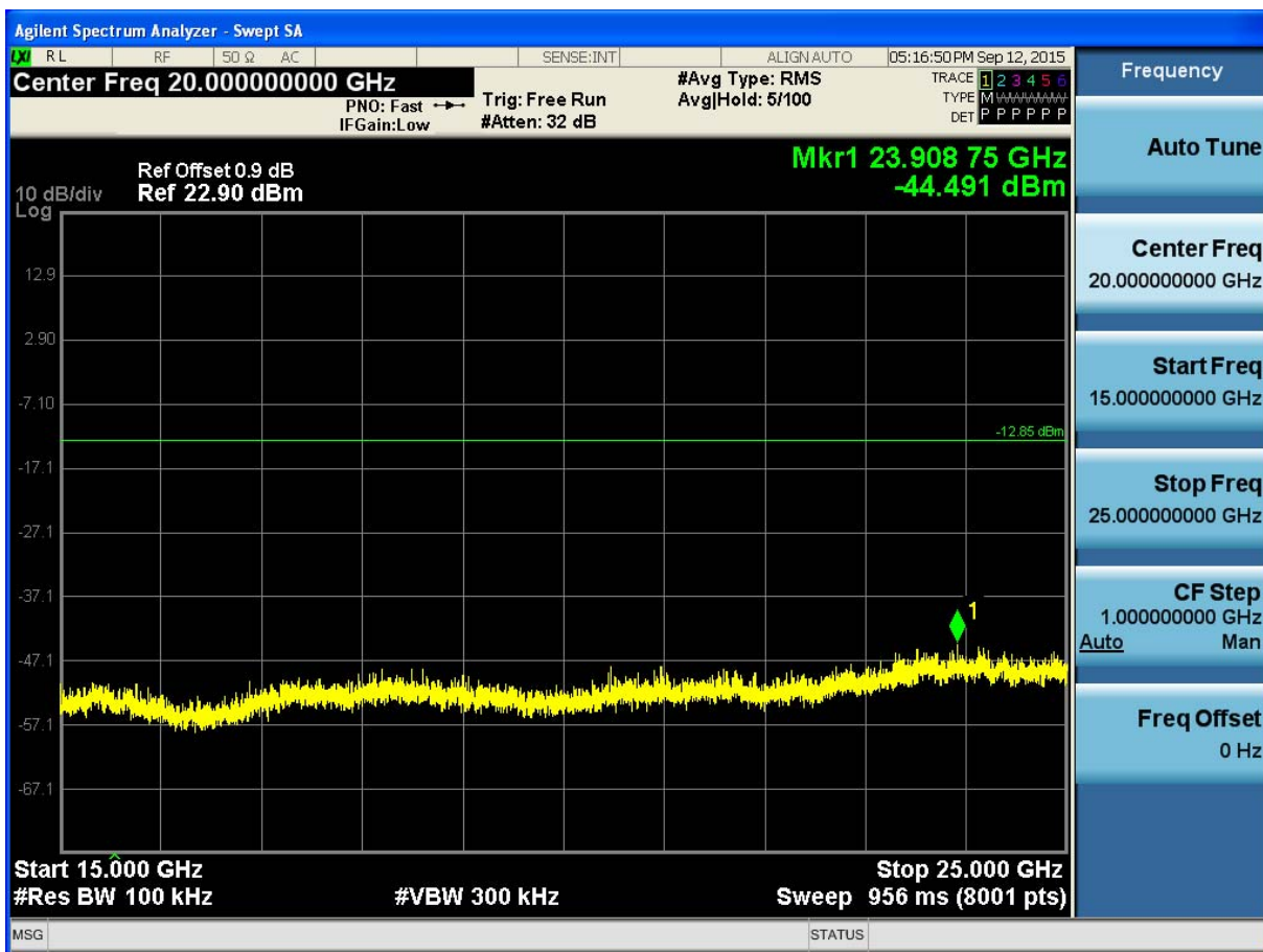
(Plot 4.6.1 C6: Channel 39: 2480MHz @ GFSK)
