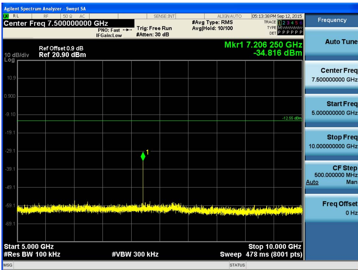
(Plot 4.6.1 A4: Channel 00: 2402MHz @ GFSK)
