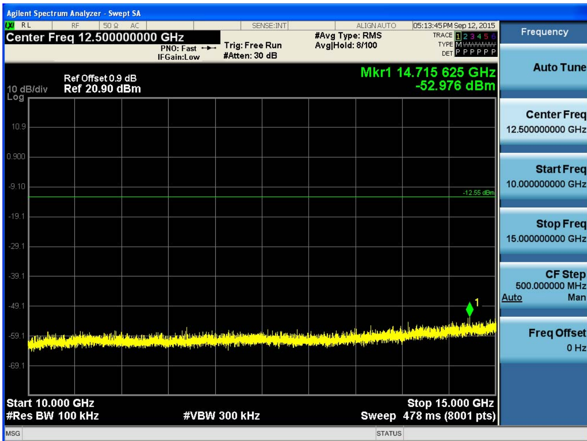
(Plot 4.6.1 A5: Channel 00: 2402MHz @ GFSK)
