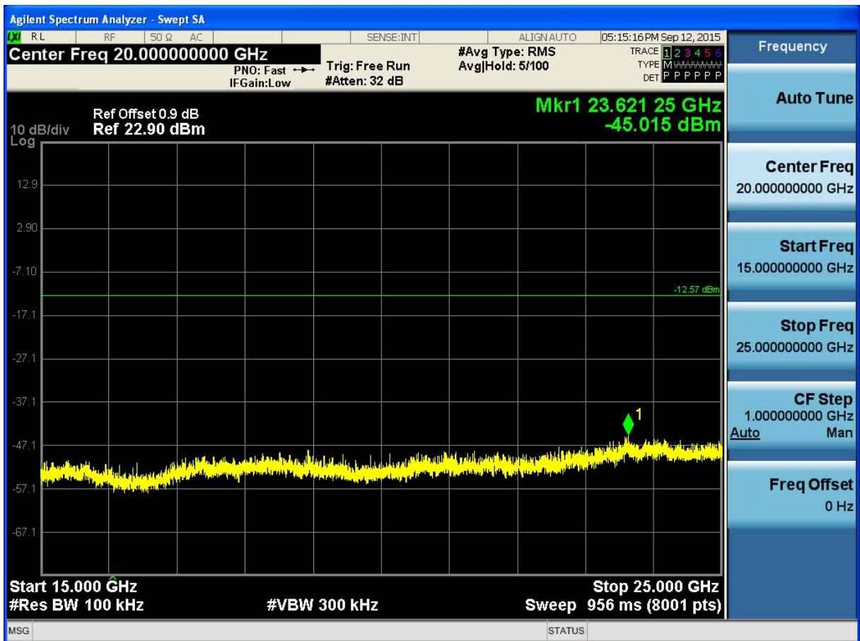
(Plot 4.6.1 B6: Channel 19: 2440MHz @ GFSK)
