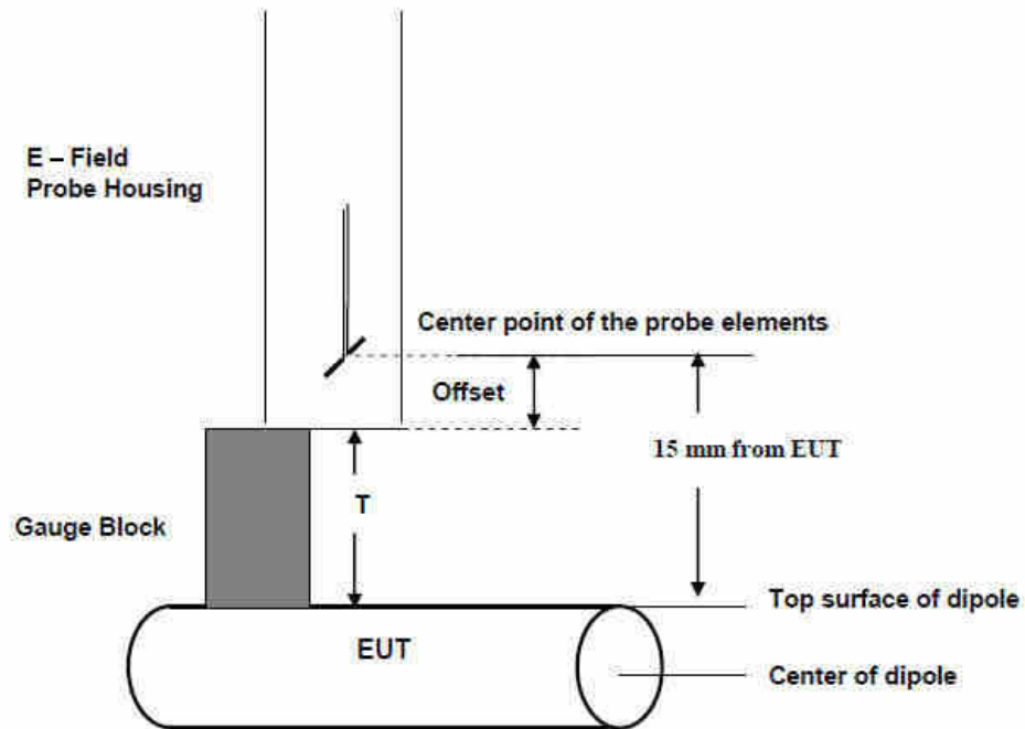
Fig. 7.3 Gauge block with E-field probe
