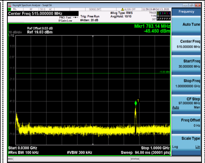
30MHz-1GHz
