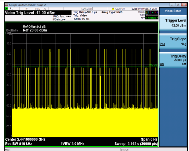
Number of bursts in 3.16s
