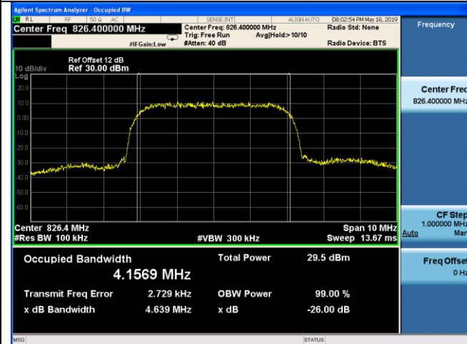
Channel 4132 / 826.4 MHz
