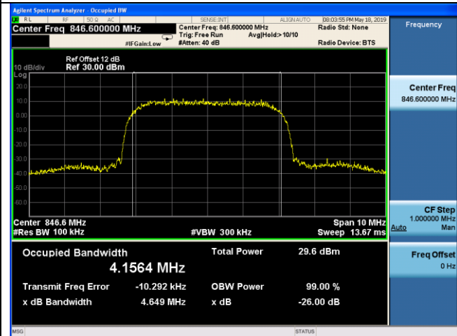
Channel 4233 / 846.6 MHz
