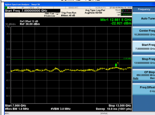
7GHz-13.5GHz
