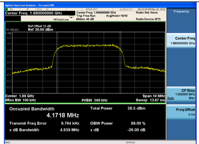
Channel 9400 / 1880.0 MHz
