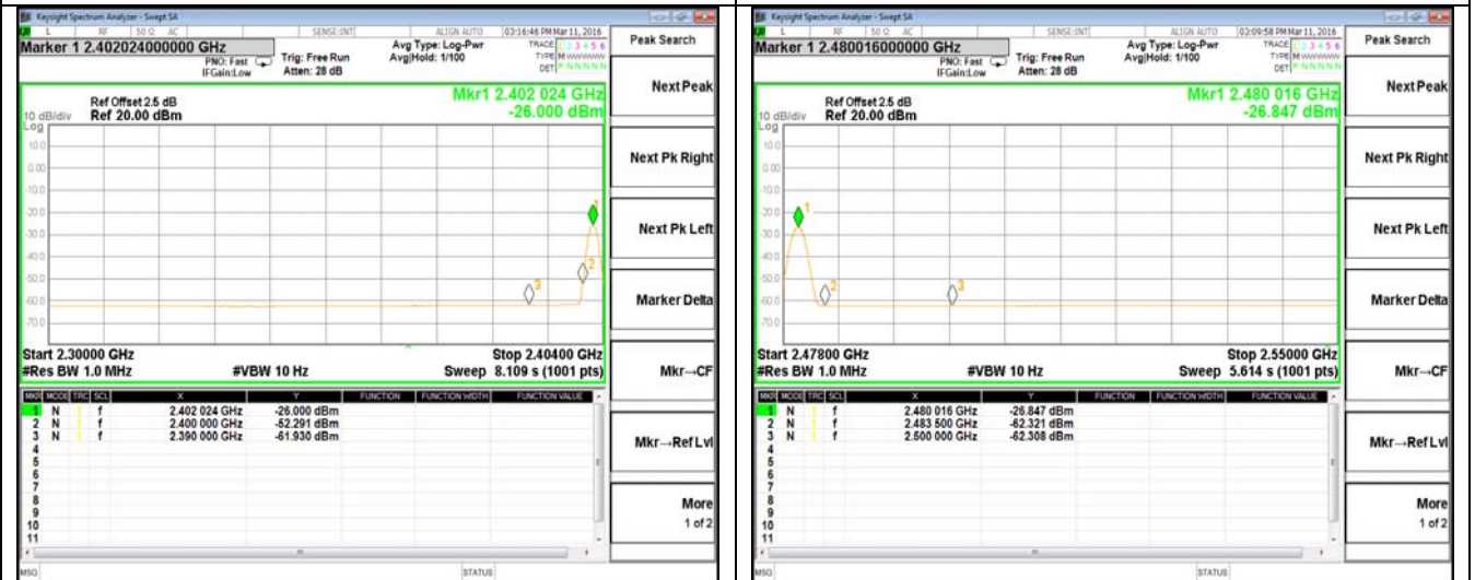
2402 MHz – Average
