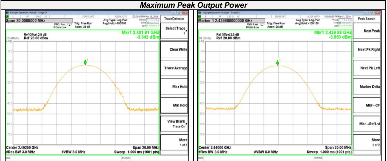
2402 MHz
