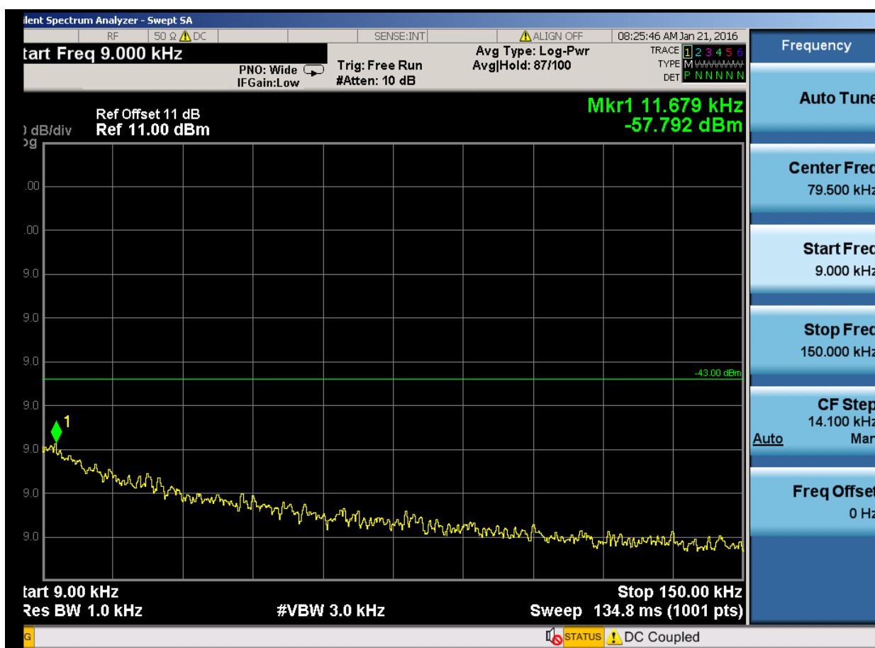
(Plot 4.5.1 A1: Channel 128: 824.20MHz @ Traffic @ GSM850)
