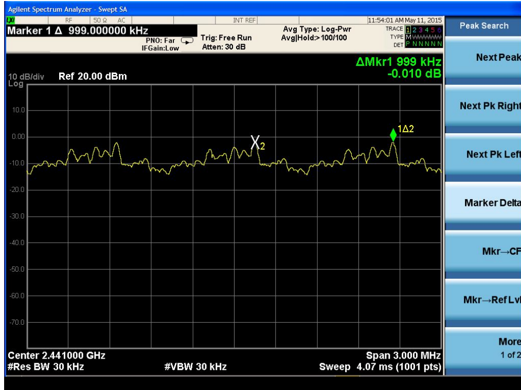
(Plot 4.6.2 A: Channel 39: 2441MHz @ 8DPSK)
