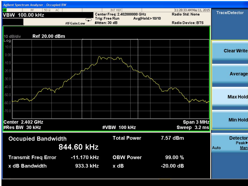
(Plot 4.4.1 A: Channel 00: 2402MHz @ GFSK)
